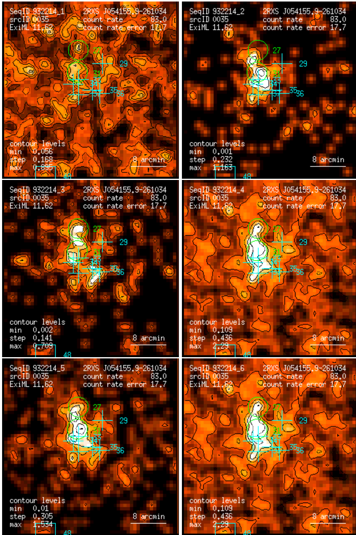
Figure 35: RASS 932214: detection 0035: band rate images, Gaussian filter: (1) PSPC channels 11 – 41, (2) 52 – 90, (3) 91 – 201, (4) 11 – 235, (5) 52 – 201, (6) 11 – 201. Broad band rates in counts/ks. Band rate contour levels in counts/ks/arcmin 2 .
