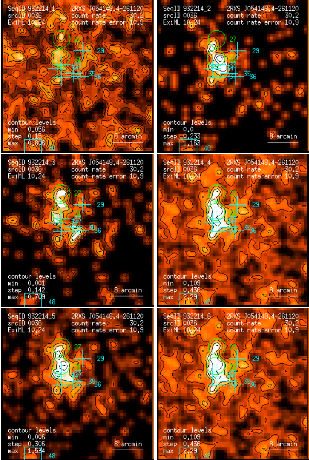
Figure 36: RASS 932214: detection 0036: band rate images, Gaussian filter: (1) PSPC channels 11 – 41, (2) 52 – 90, (3) 91 – 201, (4) 11 – 235, (5) 52 – 201, (6) 11 – 201. Broad band rates in counts/ks. Band rate contour levels in counts/ks/arcmin 2 .
