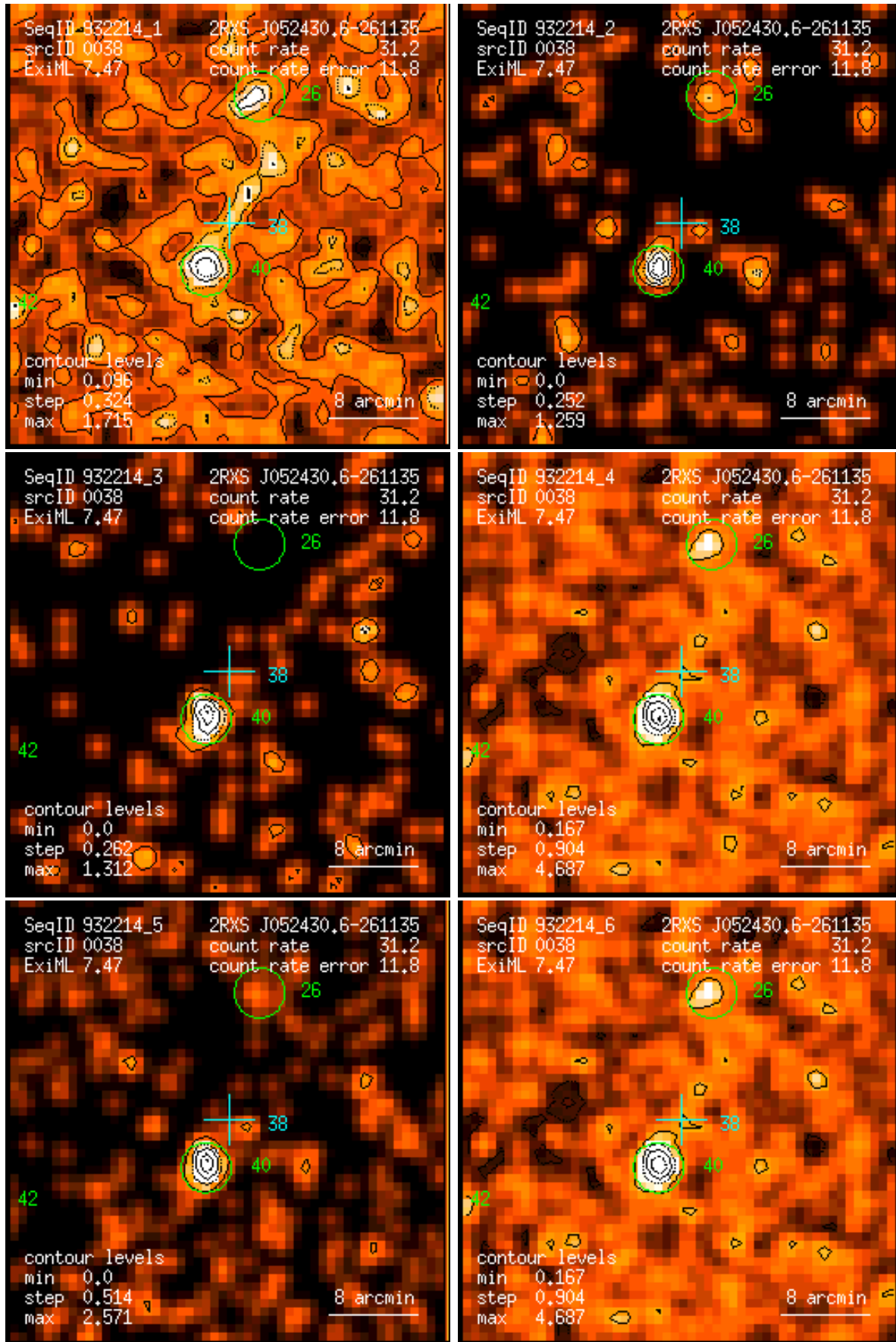
Figure 38: RASS 932214: detection 0038: band rate images, Gaussian filter: (1) PSPC channels 11 – 41, (2) 52 – 90, (3) 91 – 201, (4) 11 – 235, (5) 52 – 201, (6) 11 – 201. Broad band rates in counts/ks. Band rate contour levels in counts/ks/arcmin 2 .
