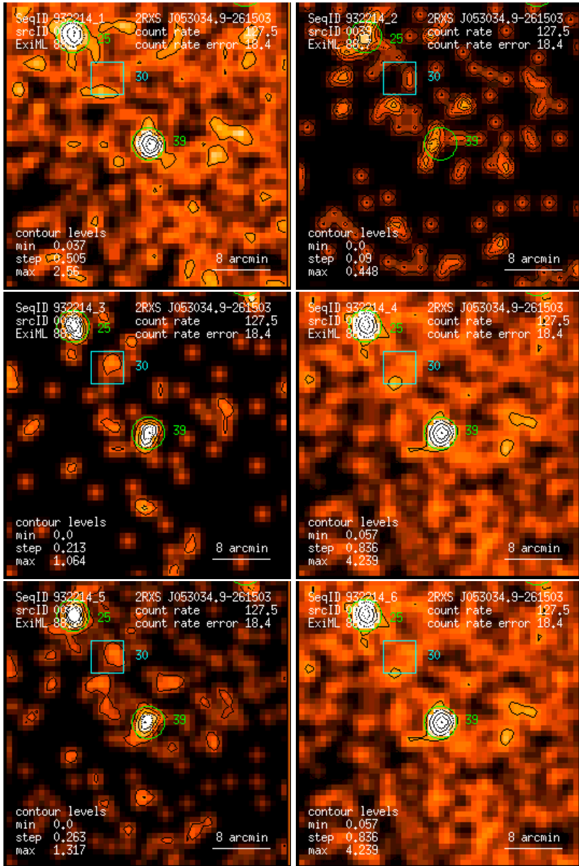
Figure 39: RASS 932214: detection 0039: band rate images, Gaussian filter: (1) PSPC channels 11 – 41, (2) 52 – 90, (3) 91 – 201, (4) 11 – 235, (5) 52 – 201, (6) 11 – 201. Broad band rates in counts/ks. Band rate contour levels in counts/ks/arcmin 2 .
