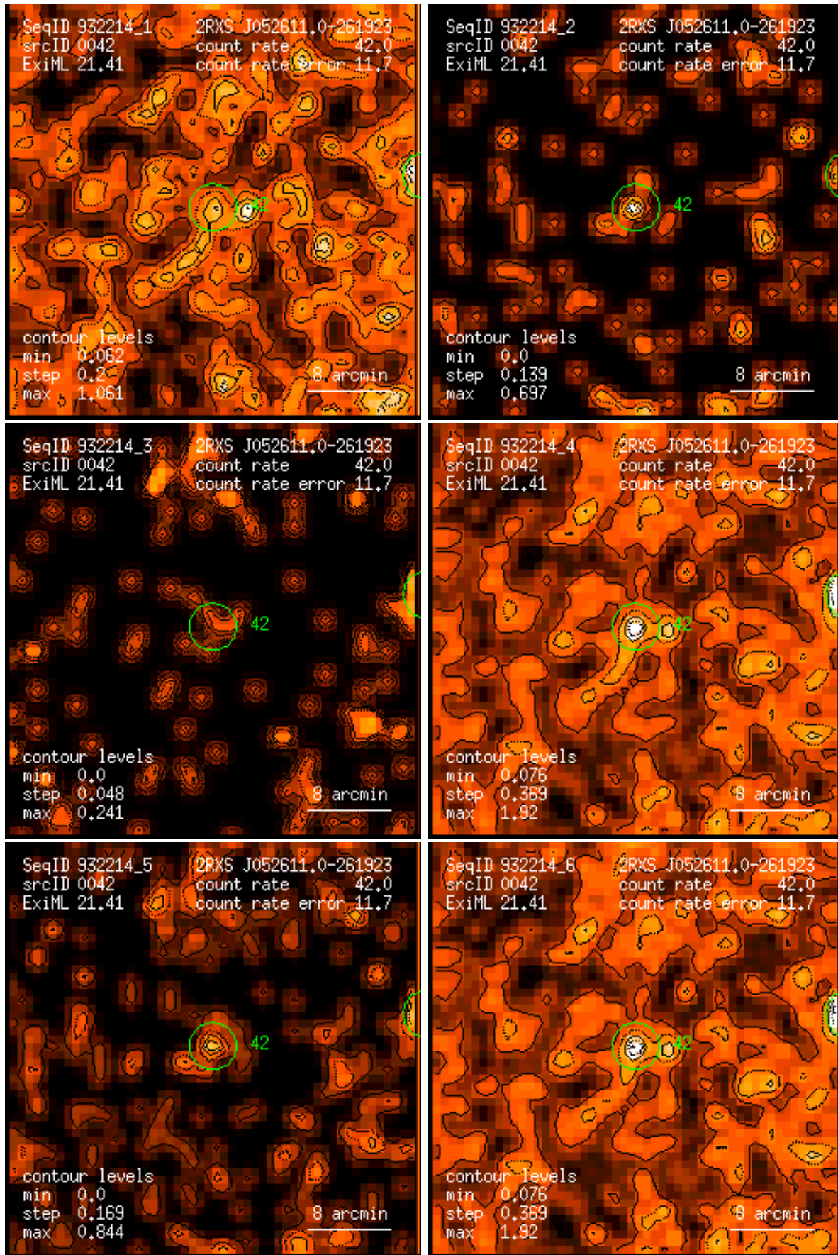
Figure 42: RASS 932214: detection 0042: band rate images, Gaussian filter: (1) PSPC channels 11 – 41, (2) 52 – 90, (3) 91 – 201, (4) 11 – 235, (5) 52 – 201, (6) 11 – 201. Broad band rates in counts/ks. Band rate contour levels in counts/ks/arcmin 2 .
