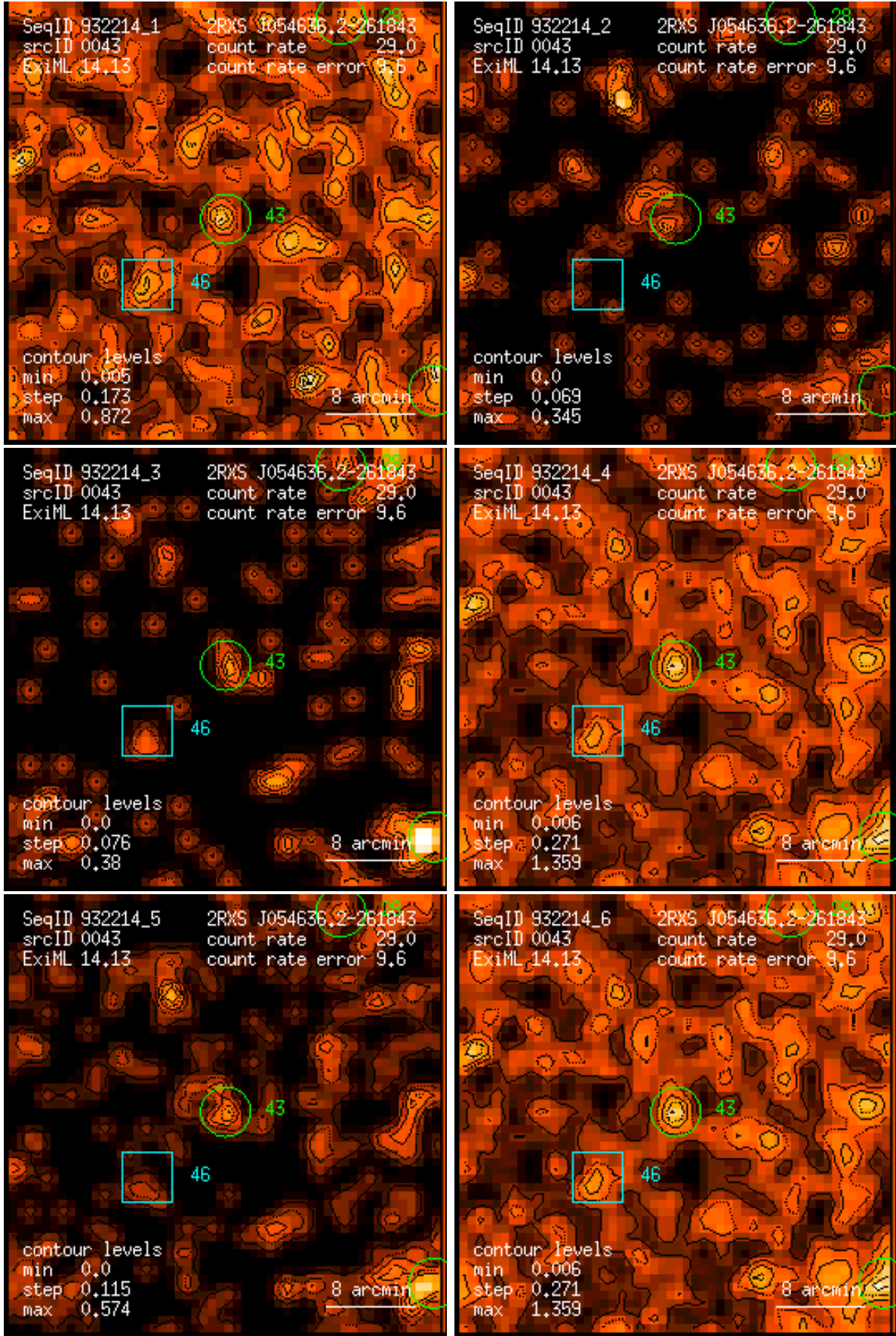
Figure 43: RASS 932214: detection 0043: band rate images, Gaussian filter: (1) PSPC channels 11 – 41, (2) 52 – 90, (3) 91 – 201, (4) 11 – 235, (5) 52 – 201, (6) 11 – 201. Broad band rates in counts/ks. Band rate contour levels in counts/ks/arcmin 2 .
