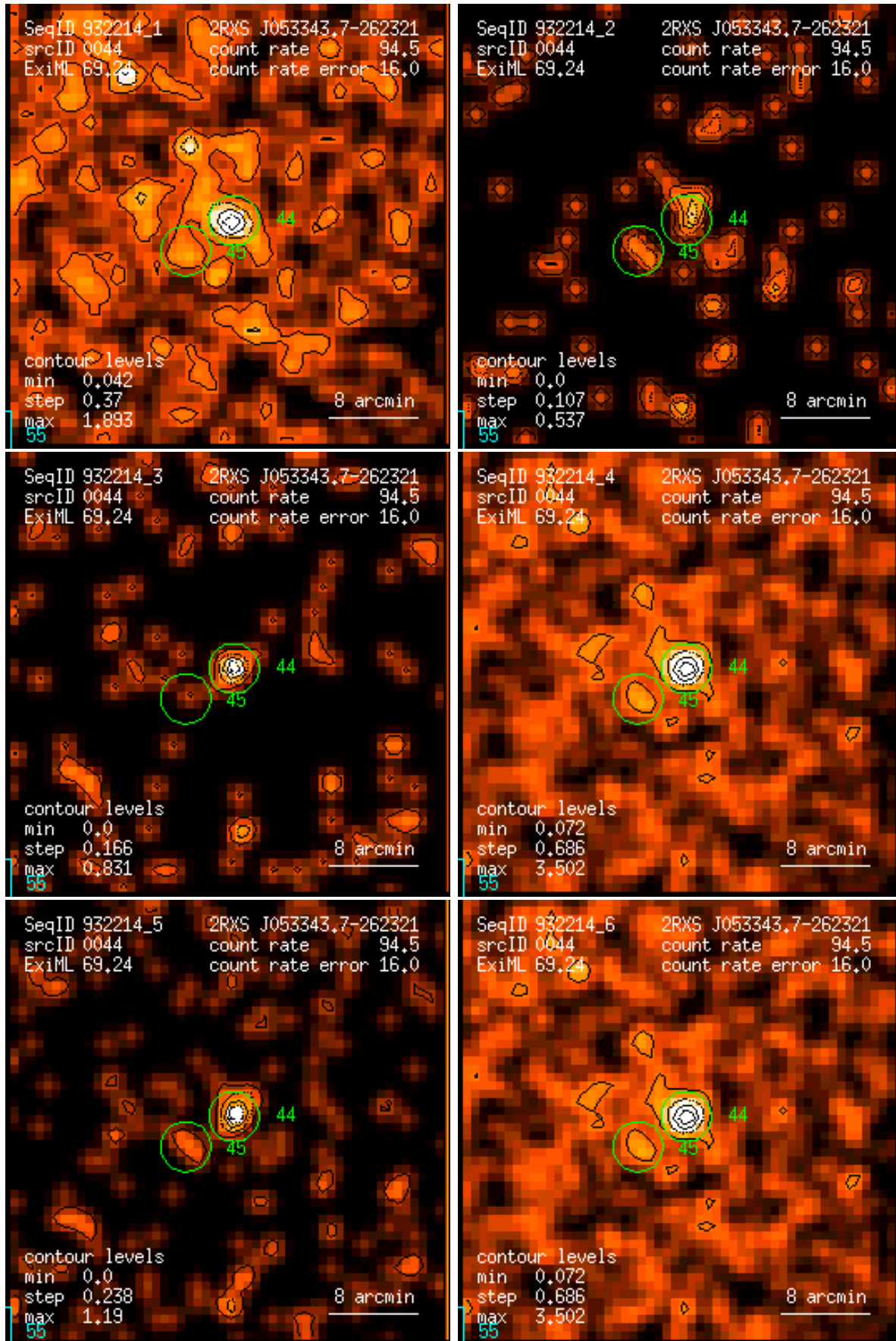
Figure 44: RASS 932214: detection 0044: band rate images, Gaussian filter: (1) PSPC channels 11 – 41, (2) 52 – 90, (3) 91 – 201, (4) 11 – 235, (5) 52 – 201, (6) 11 – 201. Broad band rates in counts/ks. Band rate contour levels in counts/ks/arcmin 2 .
