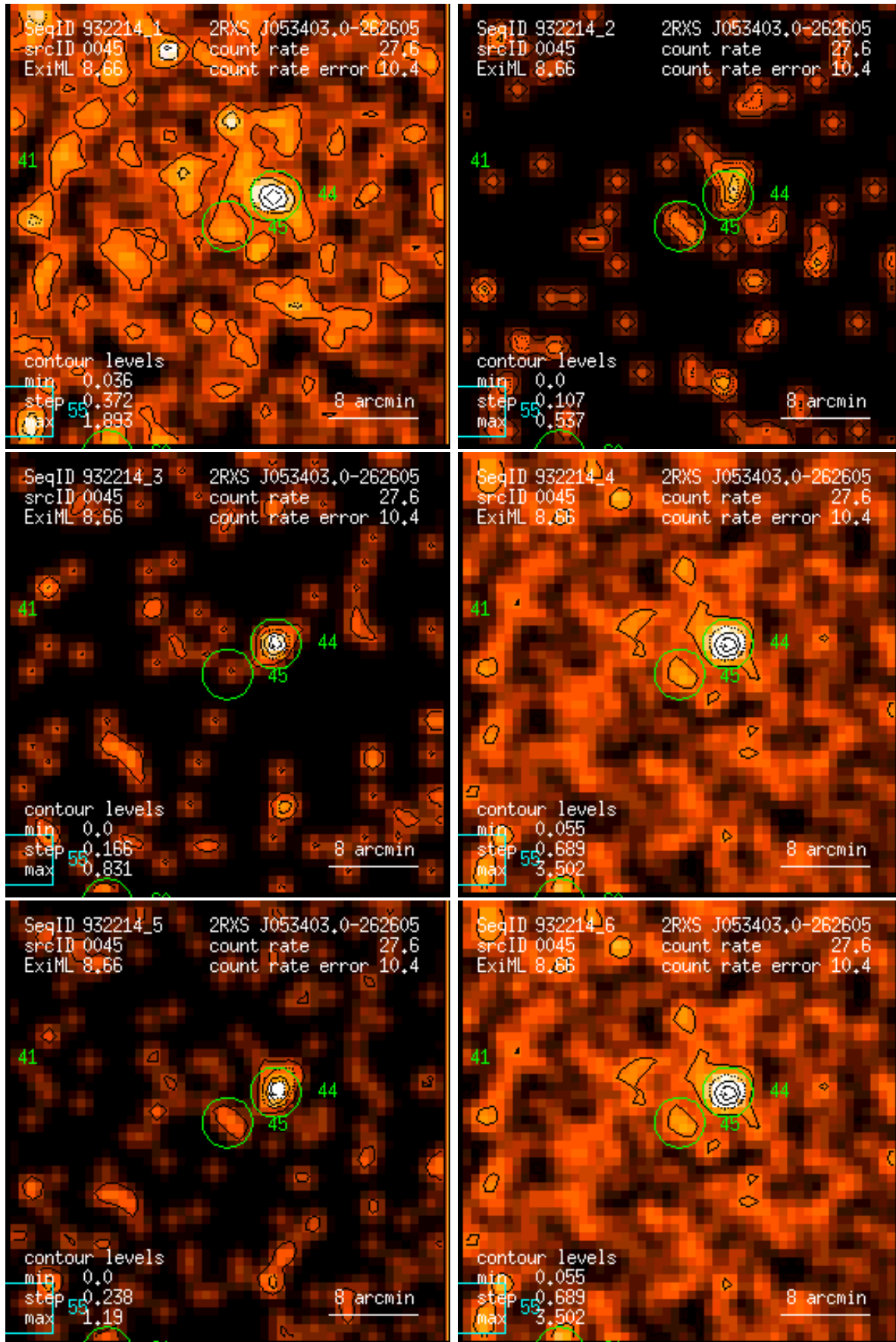
Figure 45: RASS 932214: detection 0045: band rate images, Gaussian filter: (1) PSPC channels 11 – 41, (2) 52 – 90, (3) 91 – 201, (4) 11 – 235, (5) 52 – 201, (6) 11 – 201. Broad band rates in counts/ks. Band rate contour levels in counts/ks/arcmin 2 .
