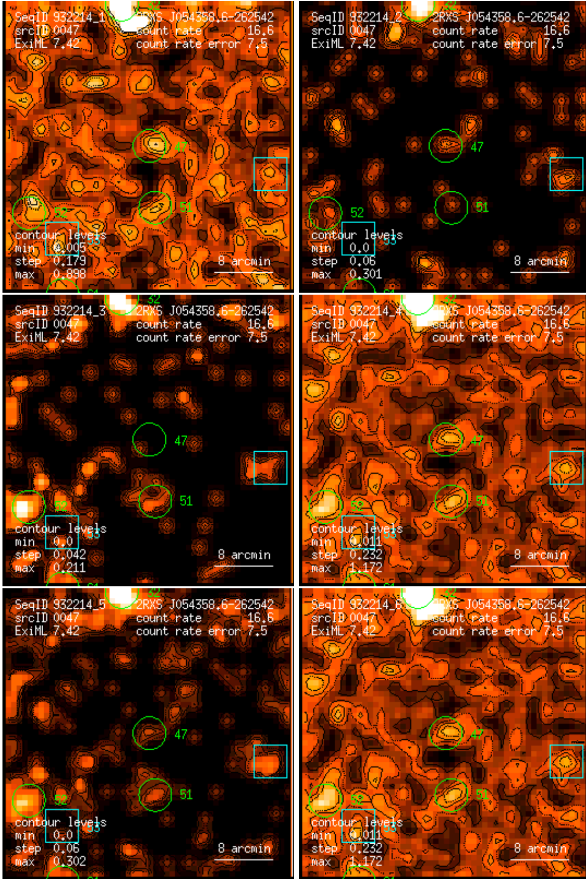
Figure 47: RASS 932214: detection 0047: band rate images, Gaussian filter: (1) PSPC channels 11 – 41, (2) 52 – 90, (3) 91 – 201, (4) 11 – 235, (5) 52 – 201, (6) 11 – 201. Broad band rates in counts/ks. Band rate contour levels in counts/ks/arcmin 2 .
