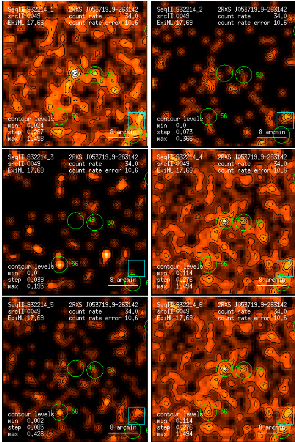
Figure 49: RASS 932214: detection 0049: band rate images, Gaussian filter: (1) PSPC channels 11 – 41, (2) 52 – 90, (3) 91 – 201, (4) 11 – 235, (5) 52 – 201, (6) 11 – 201. Broad band rates in counts/ks. Band rate contour levels in counts/ks/arcmin 2 .
