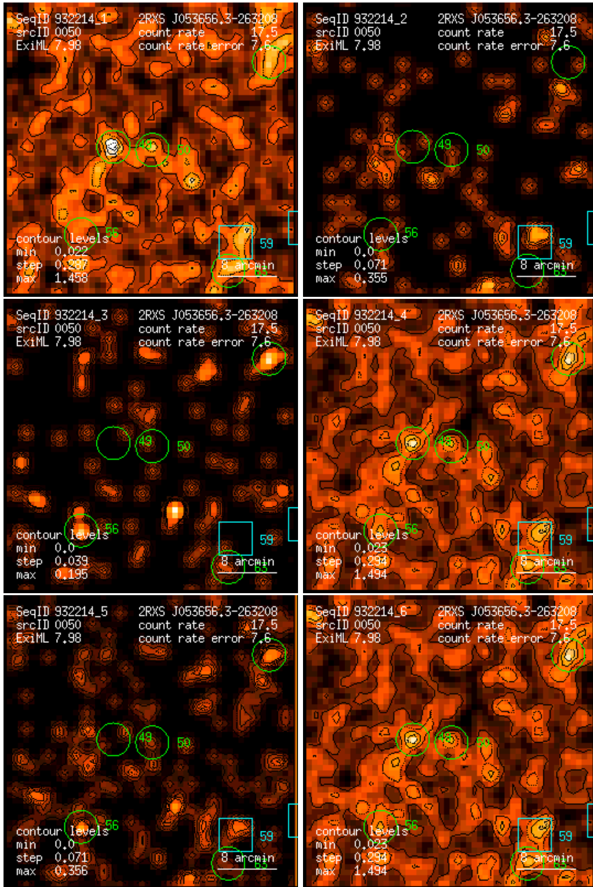
Figure 50: RASS 932214: detection 0050: band rate images, Gaussian filter: (1) PSPC channels 11 – 41, (2) 52 – 90, (3) 91 – 201, (4) 11 – 235, (5) 52 – 201, (6) 11 – 201. Broad band rates in counts/ks. Band rate contour levels in counts/ks/arcmin 2 .
