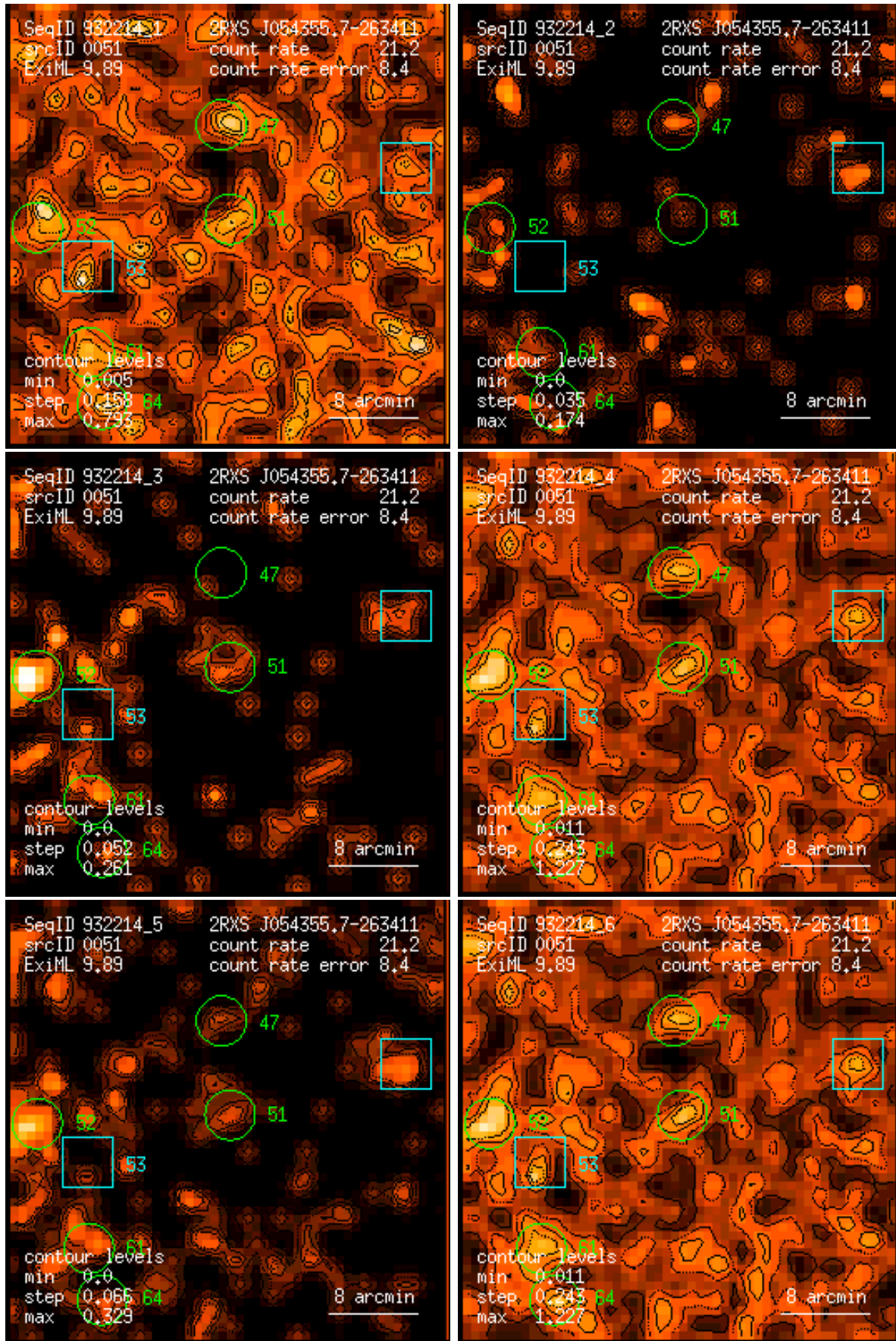
Figure 51: RASS 932214: detection 0051: band rate images, Gaussian filter: (1) PSPC channels 11 – 41, (2) 52 – 90, (3) 91 – 201, (4) 11 – 235, (5) 52 – 201, (6) 11 – 201. Broad band rates in counts/ks. Band rate contour levels in counts/ks/arcmin 2 .
