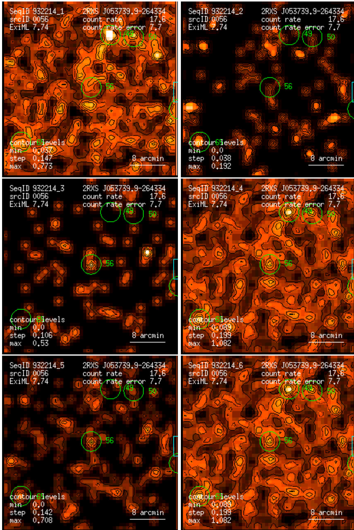
Figure 56: RASS 932214: detection 0056: band rate images, Gaussian filter: (1) PSPC channels 11 – 41, (2) 52 – 90, (3) 91 – 201, (4) 11 – 235, (5) 52 – 201, (6) 11 – 201. Broad band rates in counts/ks. Band rate contour levels in counts/ks/arcmin 2 .
