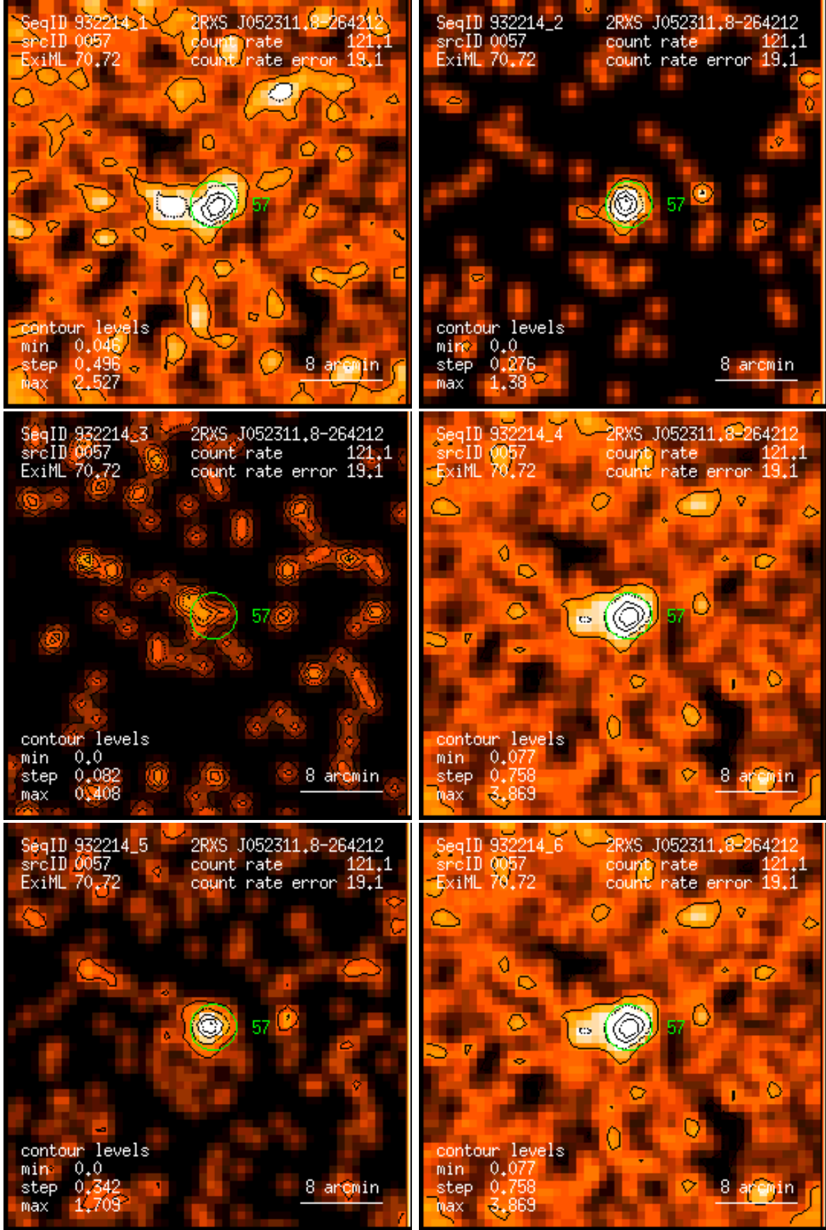
Figure 57: RASS 932214: detection 0057: band rate images, Gaussian filter: (1) PSPC channels 11 – 41, (2) 52 – 90, (3) 91 – 201, (4) 11 – 235, (5) 52 – 201, (6) 11 – 201. Broad band rates in counts/ks. Band rate contour levels in counts/ks/arcmin 2 .
