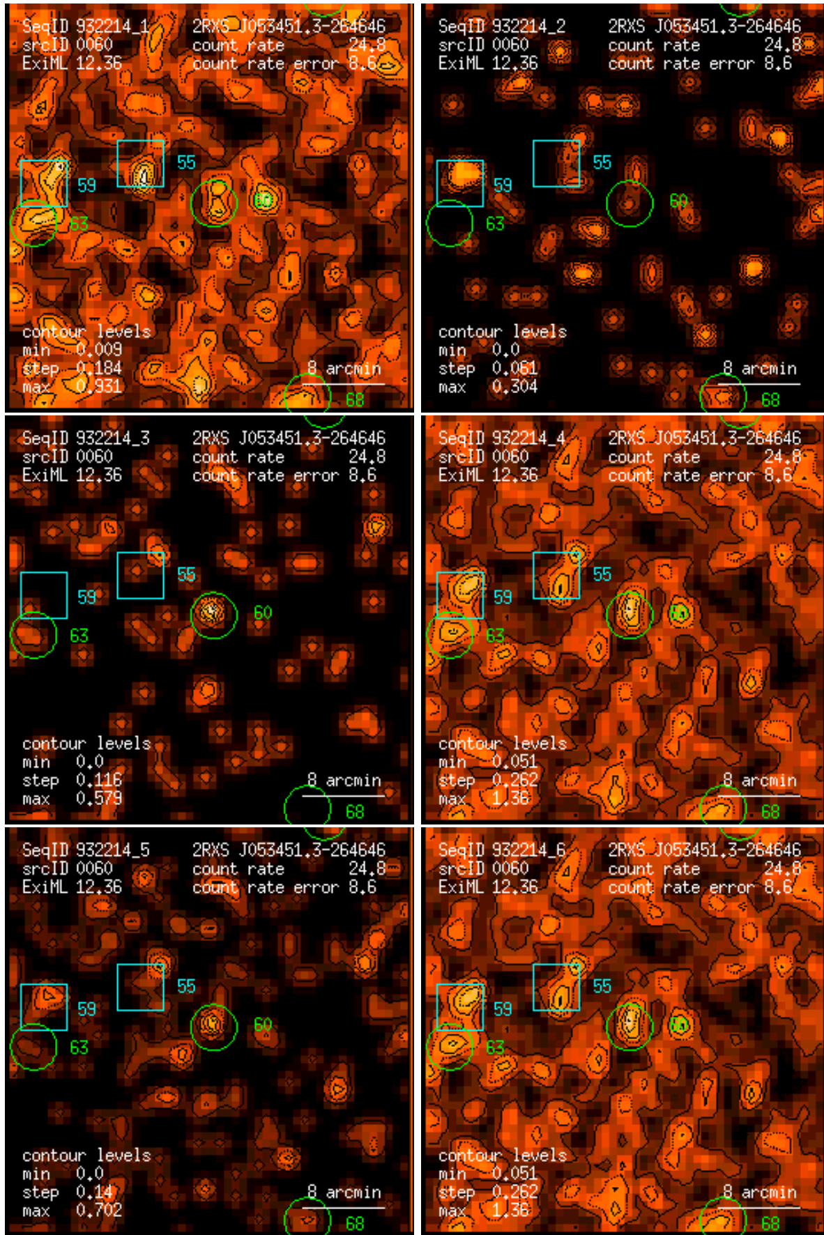
Figure 60: RASS 932214: detection 0060: band rate images, Gaussian filter: (1) PSPC channels 11 – 41, (2) 52 – 90, (3) 91 – 201, (4) 11 – 235, (5) 52 – 201, (6) 11 – 201. Broad band rates in counts/ks. Band rate contour levels in counts/ks/arcmin 2 .
