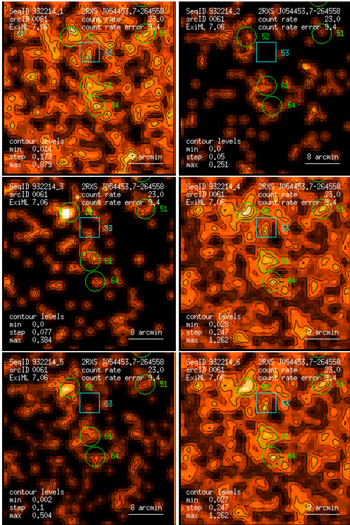
Figure 61: RASS 932214: detection 0061: band rate images, Gaussian filter: (1) PSPC channels 11 – 41, (2) 52 – 90, (3) 91 – 201, (4) 11 – 235, (5) 52 – 201, (6) 11 – 201. Broad band rates in counts/ks. Band rate contour levels in counts/ks/arcmin 2 .
