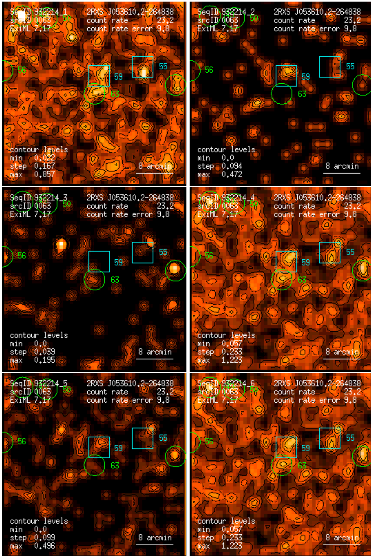
Figure 63: RASS 932214: detection 0063: band rate images, Gaussian filter: (1) PSPC channels 11 – 41, (2) 52 – 90, (3) 91 – 201, (4) 11 – 235, (5) 52 – 201, (6) 11 – 201. Broad band rates in counts/ks. Band rate contour levels in counts/ks/arcmin 2 .
