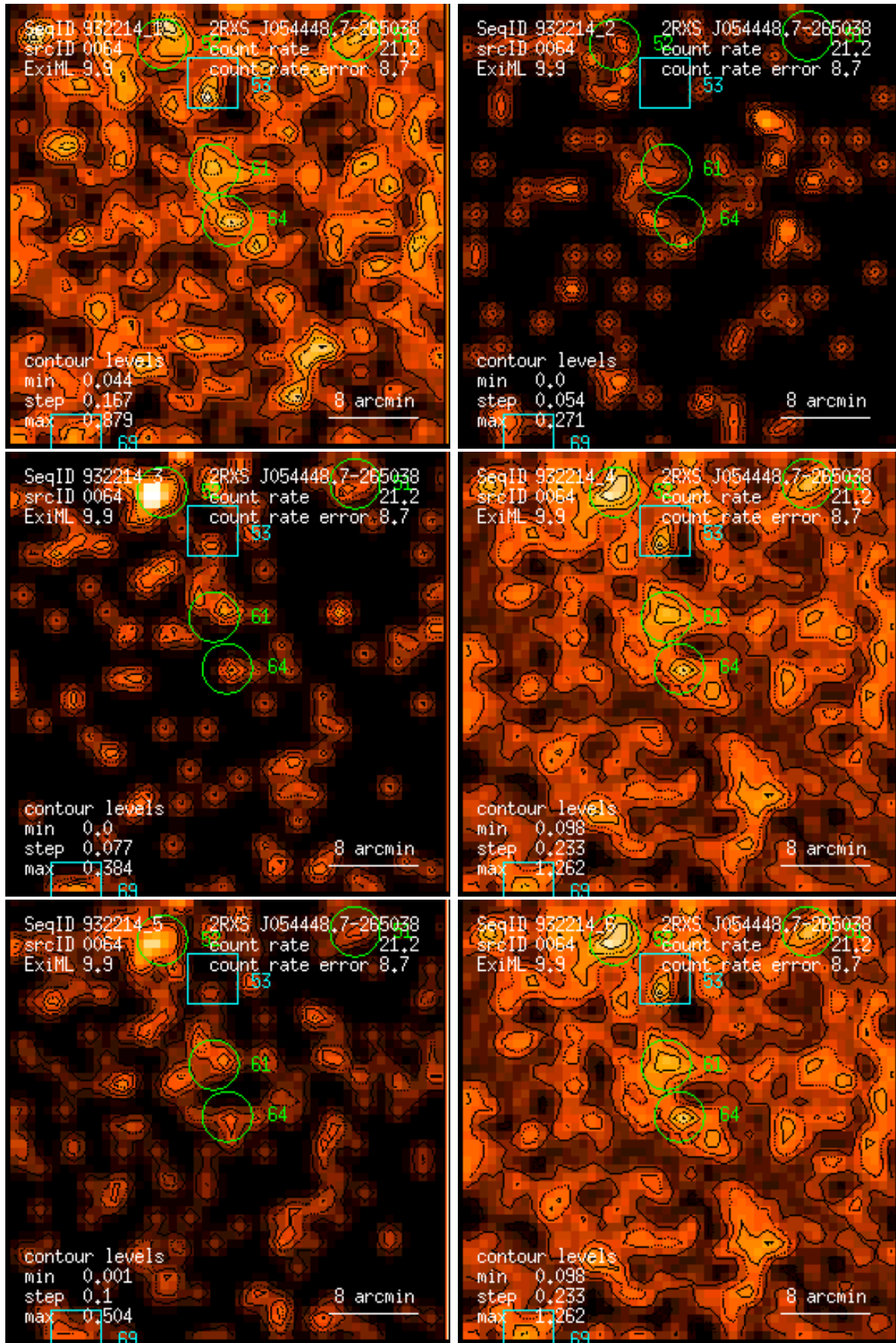
Figure 64: RASS 932214: detection 0064: band rate images, Gaussian filter: (1) PSPC channels 11 – 41, (2) 52 – 90, (3) 91 – 201, (4) 11 – 235, (5) 52 – 201, (6) 11 – 201. Broad band rates in counts/ks. Band rate contour levels in counts/ks/arcmin 2 .
