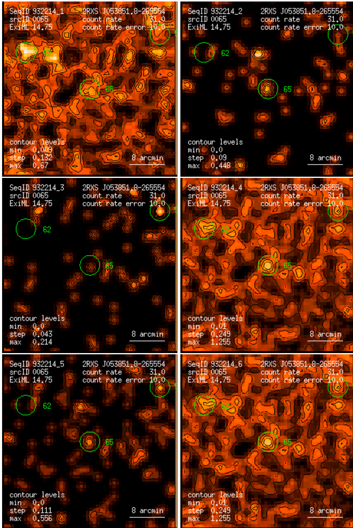
Figure 65: RASS 932214: detection 0065: band rate images, Gaussian filter: (1) PSPC channels 11 – 41, (2) 52 – 90, (3) 91 – 201, (4) 11 – 235, (5) 52 – 201, (6) 11 – 201. Broad band rates in counts/ks. Band rate contour levels in counts/ks/arcmin 2 .
