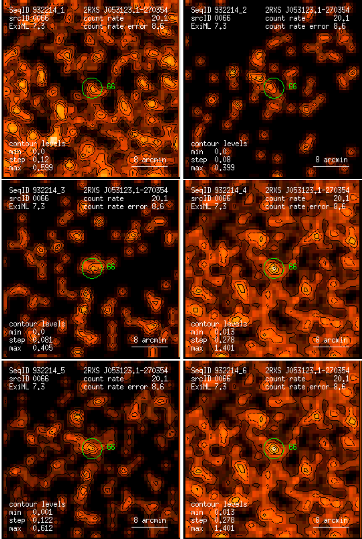
Figure 66: RASS 932214: detection 0066: band rate images, Gaussian filter: (1) PSPC channels 11 – 41, (2) 52 – 90, (3) 91 – 201, (4) 11 – 235, (5) 52 – 201, (6) 11 – 201. Broad band rates in counts/ks. Band rate contour levels in counts/ks/arcmin 2 .
