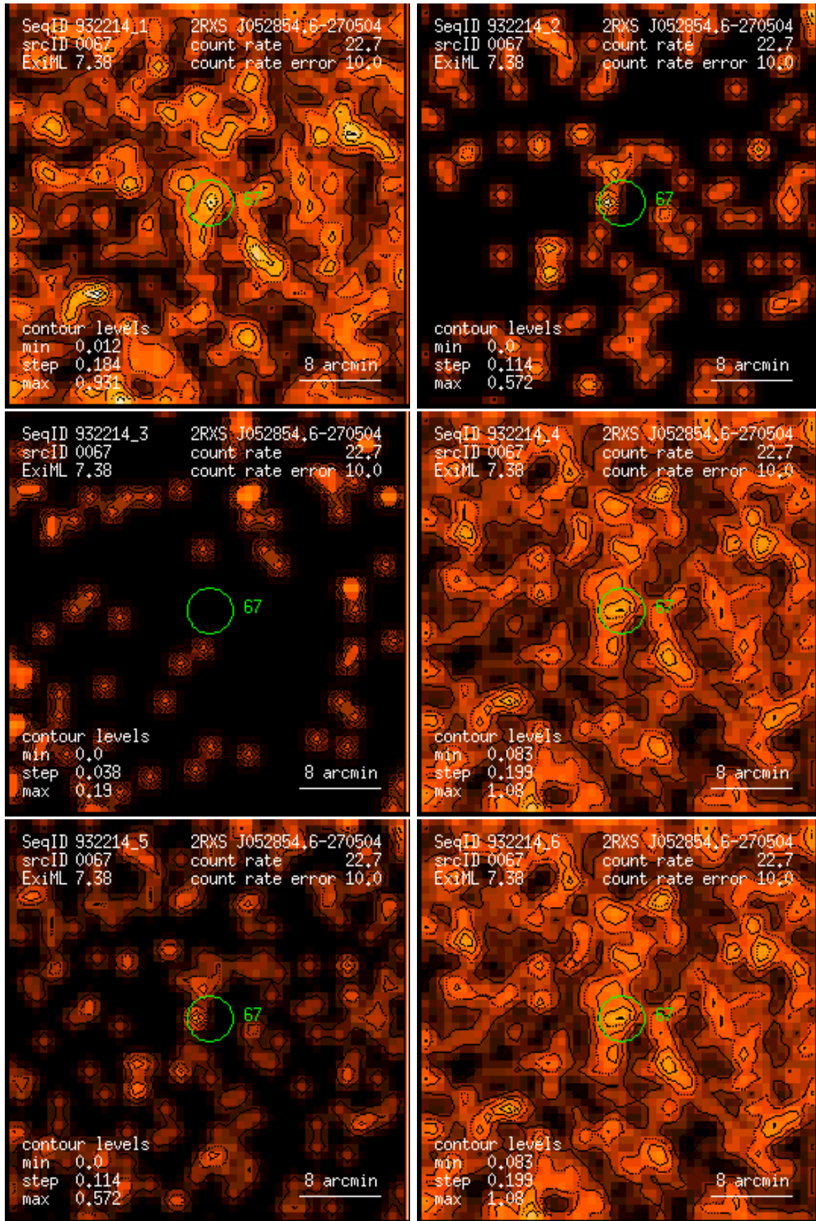
Figure 67: RASS 932214: detection 0067: band rate images, Gaussian filter: (1) PSPC channels 11 – 41, (2) 52 – 90, (3) 91 – 201, (4) 11 – 235, (5) 52 – 201, (6) 11 – 201. Broad band rates in counts/ks. Band rate contour levels in counts/ks/arcmin 2 .
