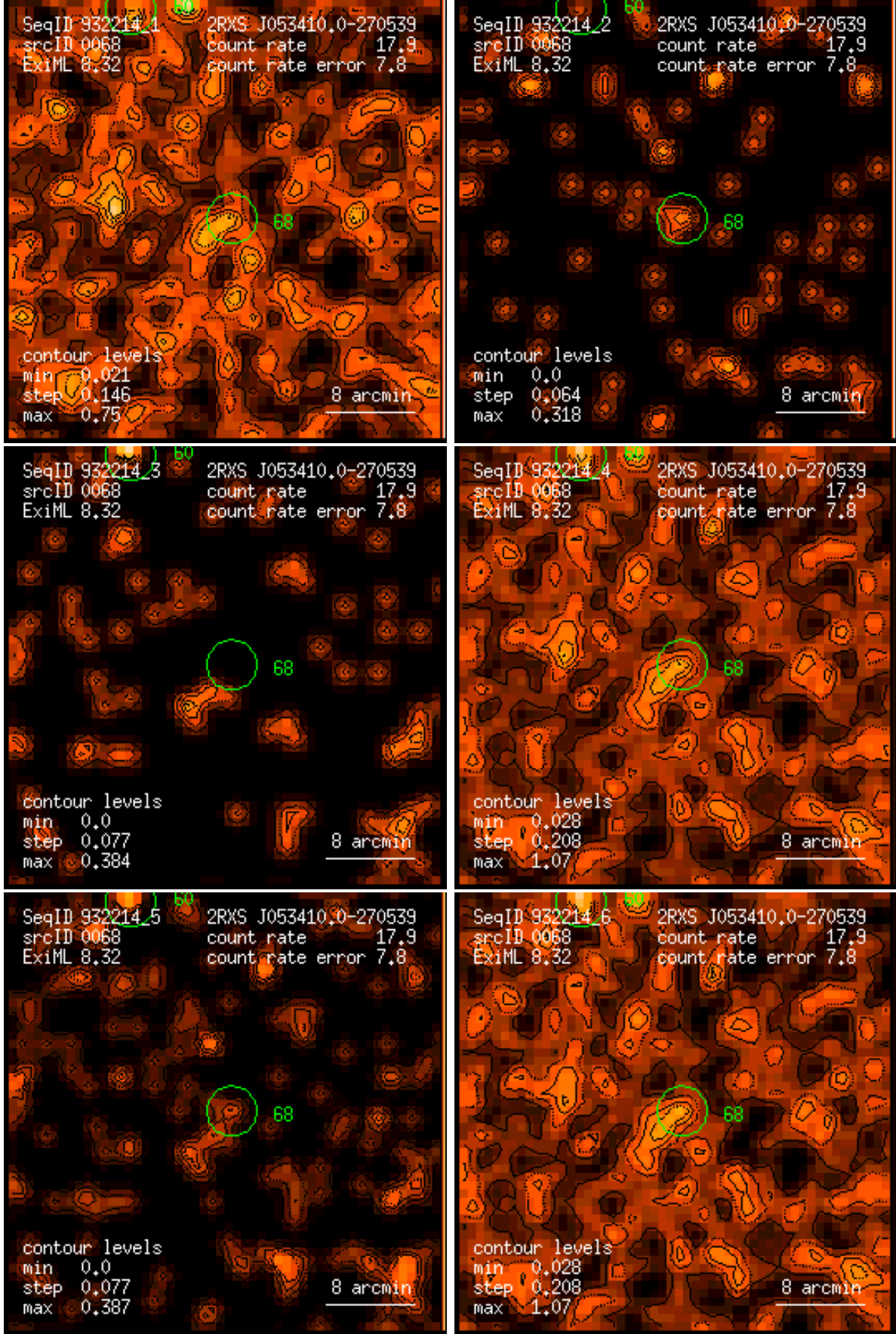
Figure 68: RASS 932214: detection 0068: band rate images, Gaussian filter: (1) PSPC channels 11 – 41, (2) 52 – 90, (3) 91 – 201, (4) 11 – 235, (5) 52 – 201, (6) 11 – 201. Broad band rates in counts/ks. Band rate contour levels in counts/ks/arcmin 2 .
