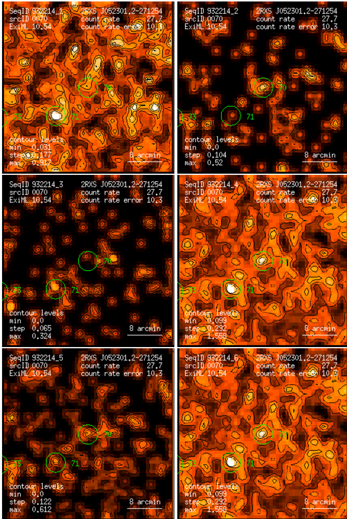
Figure 70: RASS 932214: detection 0070: band rate images, Gaussian filter: (1) PSPC channels 11 – 41, (2) 52 – 90, (3) 91 – 201, (4) 11 – 235, (5) 52 – 201, (6) 11 – 201. Broad band rates in counts/ks. Band rate contour levels in counts/ks/arcmin 2 .
