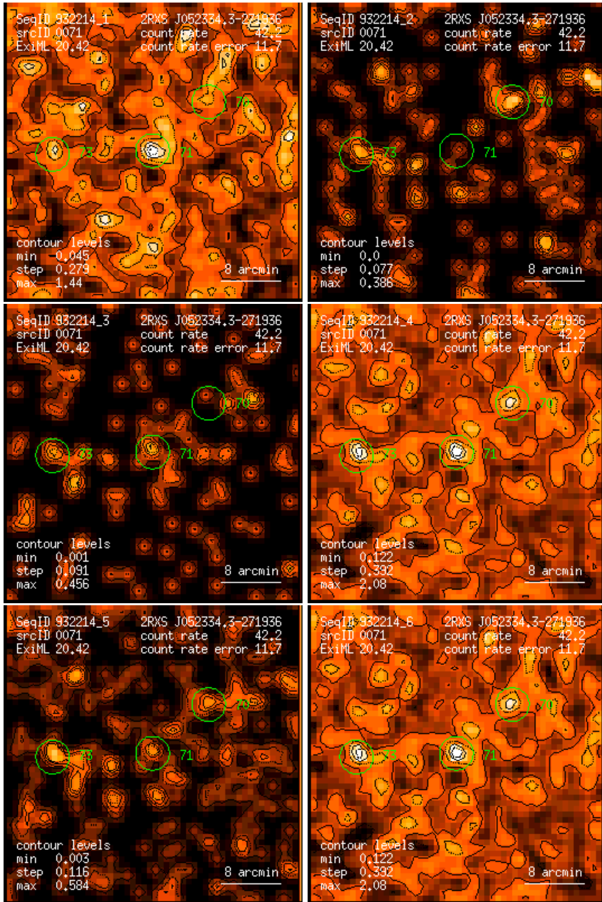
Figure 71: RASS 932214: detection 0071: band rate images, Gaussian filter: (1) PSPC channels 11 – 41, (2) 52 – 90, (3) 91 – 201, (4) 11 – 235, (5) 52 – 201, (6) 11 – 201. Broad band rates in counts/ks. Band rate contour levels in counts/ks/arcmin 2 .
