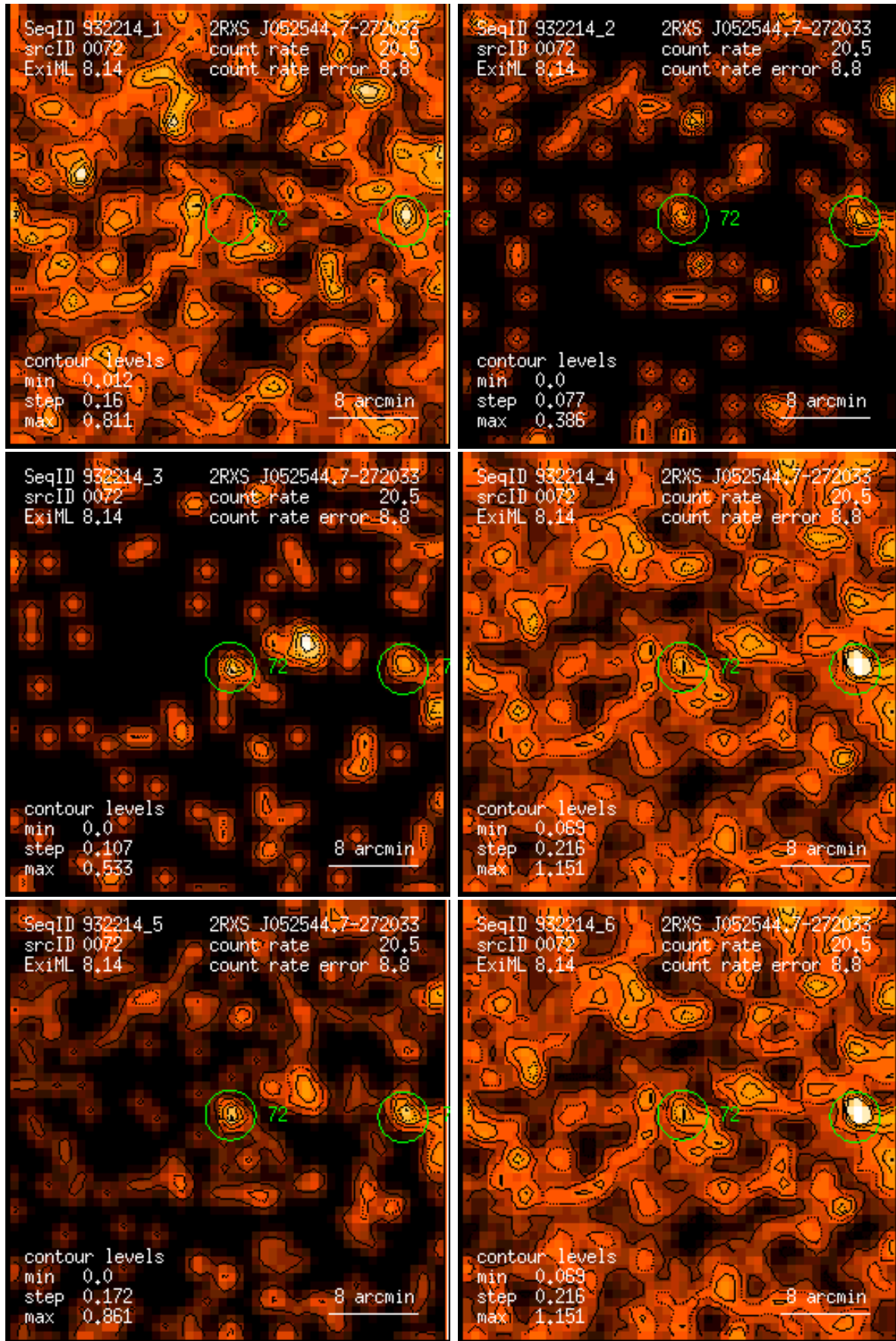
Figure 72: RASS 932214: detection 0072: band rate images, Gaussian filter: (1) PSPC channels 11 – 41, (2) 52 – 90, (3) 91 – 201, (4) 11 – 235, (5) 52 – 201, (6) 11 – 201. Broad band rates in counts/ks. Band rate contour levels in counts/ks/arcmin 2 .
