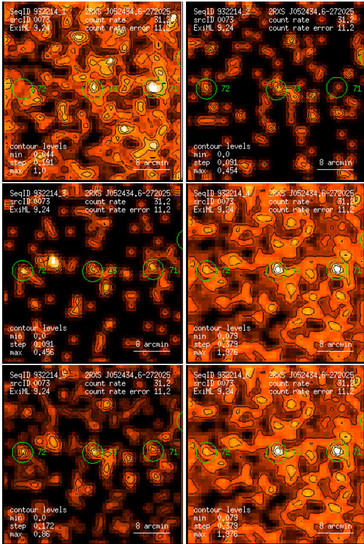
Figure 73: RASS 932214: detection 0073: band rate images, Gaussian filter: (1) PSPC channels 11 – 41, (2) 52 – 90, (3) 91 – 201, (4) 11 – 235, (5) 52 – 201, (6) 11 – 201. Broad band rates in counts/ks. Band rate contour levels in counts/ks/arcmin 2 .
