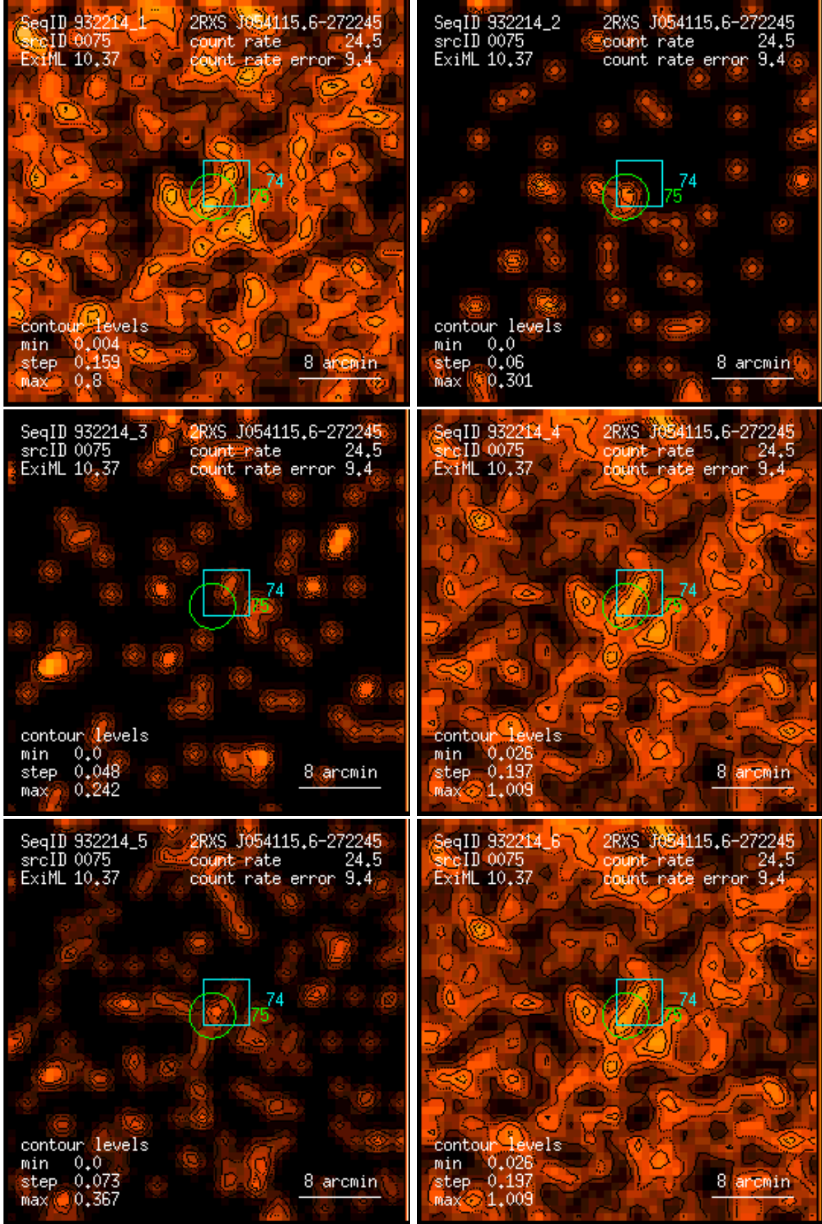
Figure 75: RASS 932214: detection 0075: band rate images, Gaussian filter: (1) PSPC channels 11 – 41, (2) 52 – 90, (3) 91 – 201, (4) 11 – 235, (5) 52 – 201, (6) 11 – 201. Broad band rates in counts/ks. Band rate contour levels in counts/ks/arcmin 2 .
