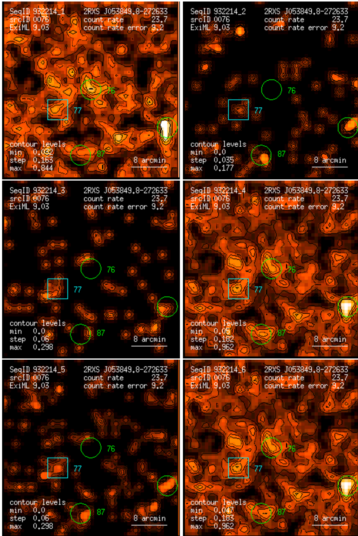
Figure 76: RASS 932214: detection 0076: band rate images, Gaussian filter: (1) PSPC channels 11 – 41, (2) 52 – 90, (3) 91 – 201, (4) 11 – 235, (5) 52 – 201, (6) 11 – 201. Broad band rates in counts/ks. Band rate contour levels in counts/ks/arcmin 2 .
