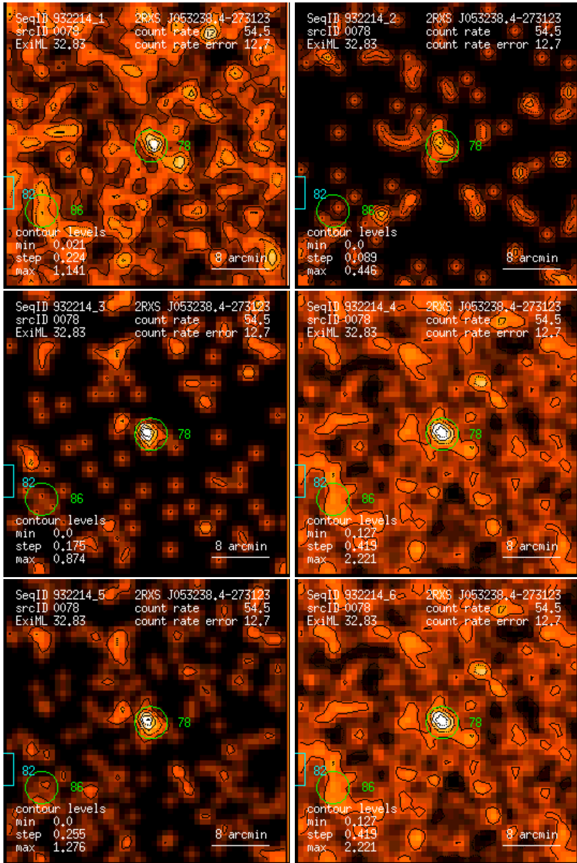
Figure 78: RASS 932214: detection 0078: band rate images, Gaussian filter: (1) PSPC channels 11 – 41, (2) 52 – 90, (3) 91 – 201, (4) 11 – 235, (5) 52 – 201, (6) 11 – 201. Broad band rates in counts/ks. Band rate contour levels in counts/ks/arcmin 2 .
