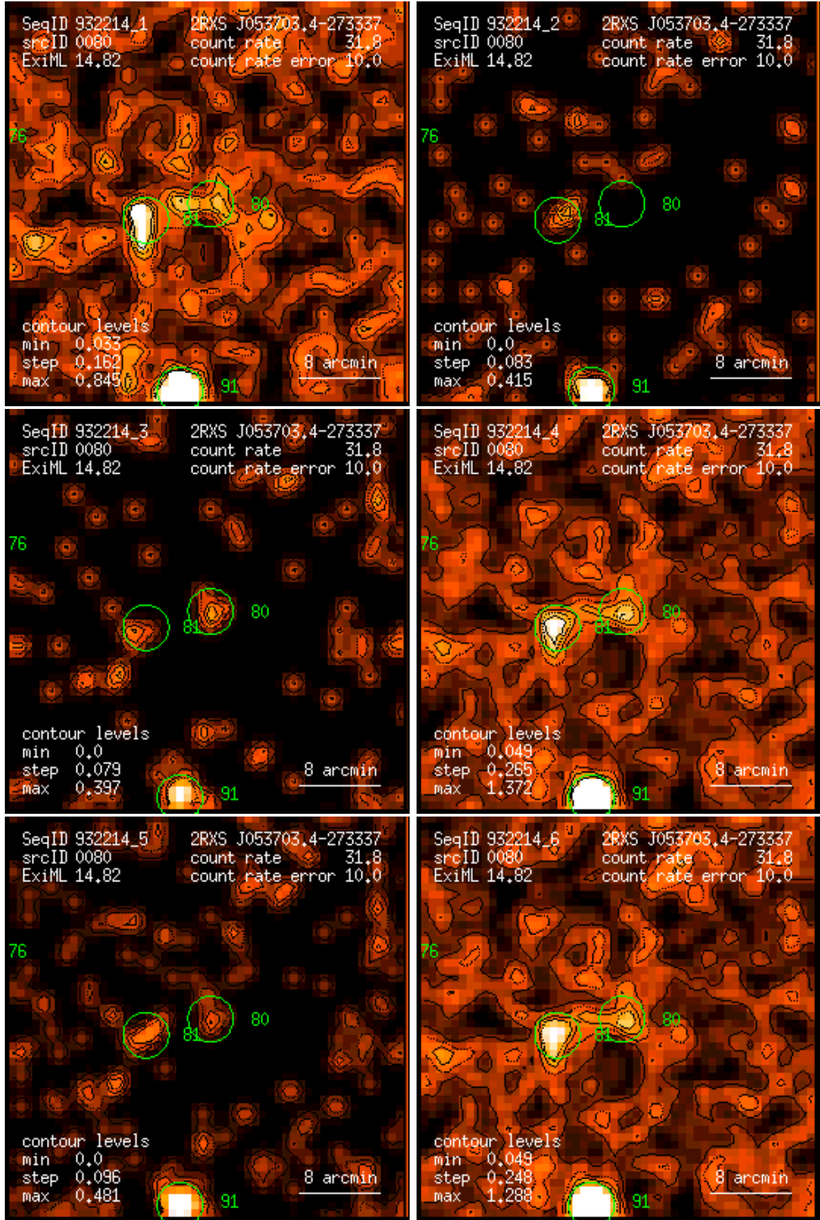
Figure 80: RASS 932214: detection 0080: band rate images, Gaussian filter: (1) PSPC channels 11 – 41, (2) 52 – 90, (3) 91 – 201, (4) 11 – 235, (5) 52 – 201, (6) 11 – 201. Broad band rates in counts/ks. Band rate contour levels in counts/ks/arcmin 2 .
