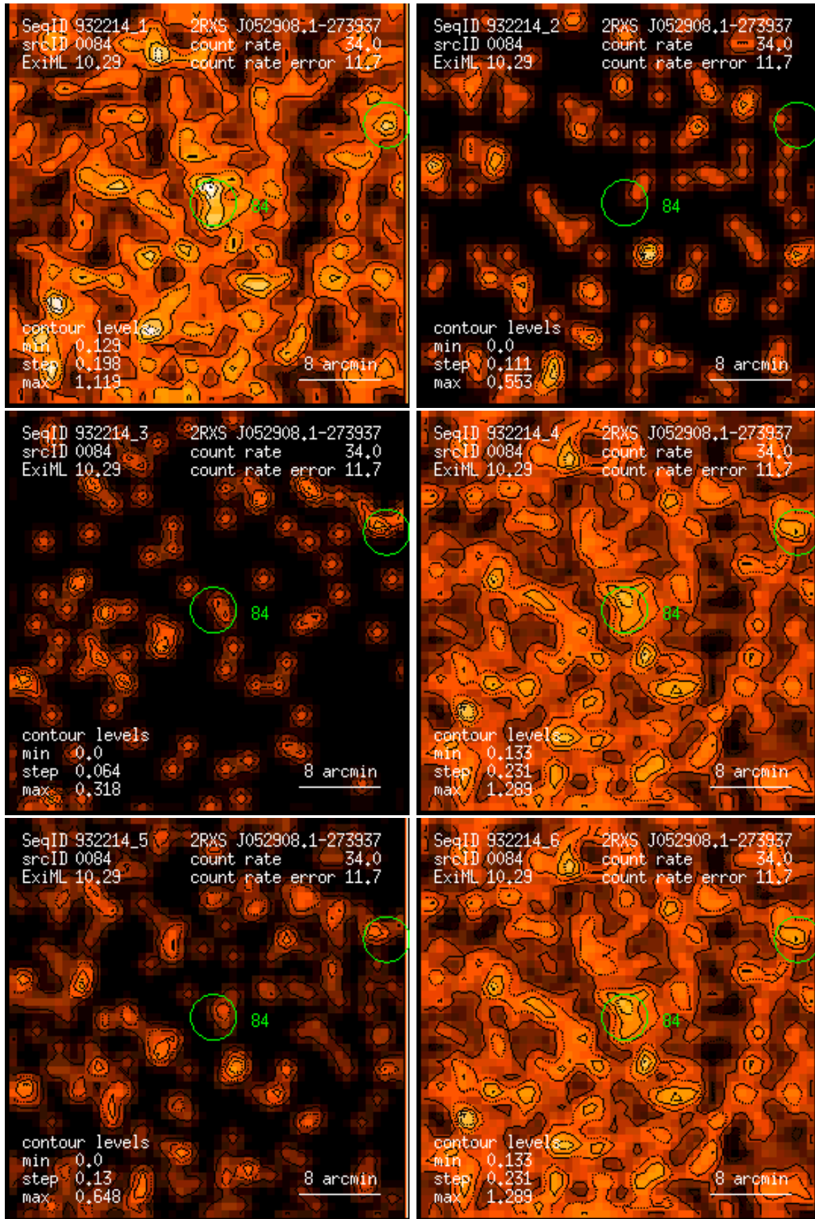
Figure 84: RASS 932214: detection 0084: band rate images, Gaussian filter: (1) PSPC channels 11 – 41, (2) 52 – 90, (3) 91 – 201, (4) 11 – 235, (5) 52 – 201, (6) 11 – 201. Broad band rates in counts/ks. Band rate contour levels in counts/ks/arcmin 2 .
