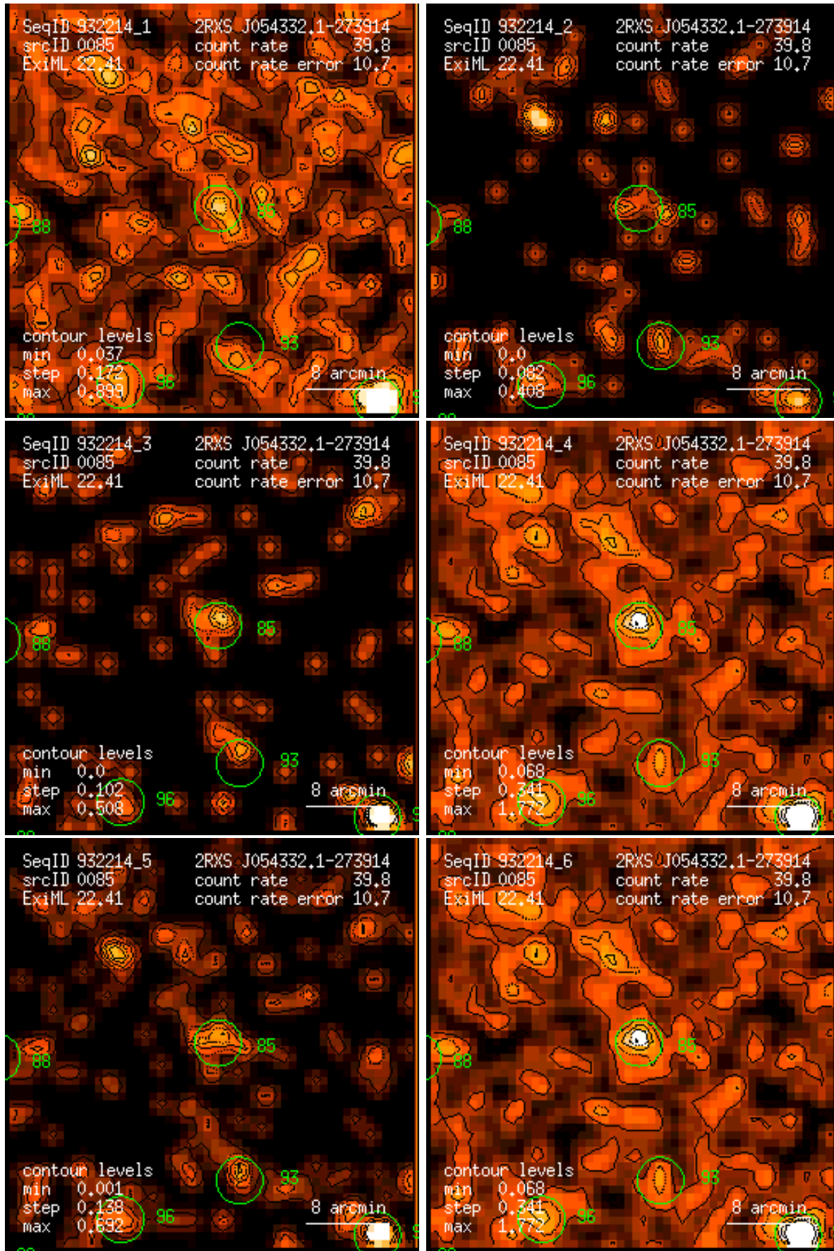
Figure 85: RASS 932214: detection 0085: band rate images, Gaussian filter: (1) PSPC channels 11 – 41, (2) 52 – 90, (3) 91 – 201, (4) 11 – 235, (5) 52 – 201, (6) 11 – 201. Broad band rates in counts/ks. Band rate contour levels in counts/ks/arcmin 2 .
