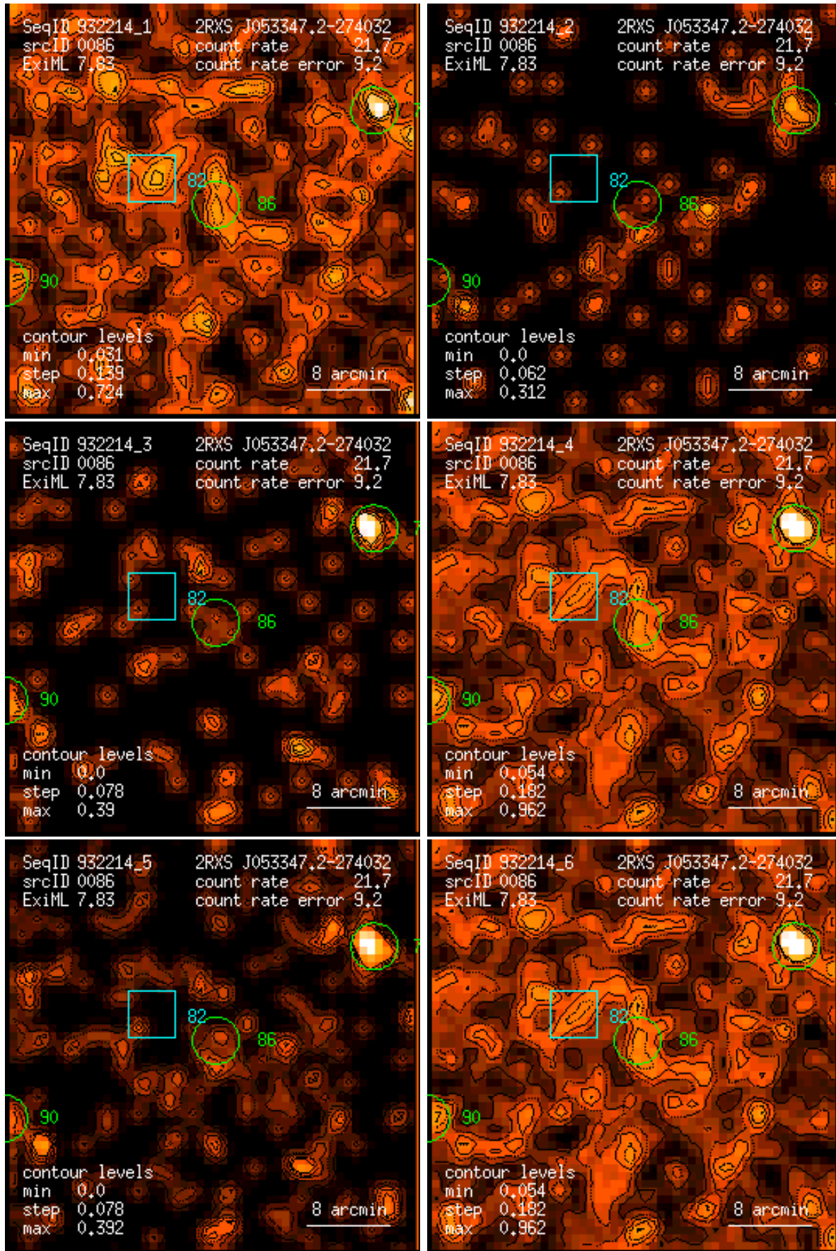
Figure 86: RASS 932214: detection 0086: band rate images, Gaussian filter: (1) PSPC channels 11 – 41, (2) 52 – 90, (3) 91 – 201, (4) 11 – 235, (5) 52 – 201, (6) 11 – 201. Broad band rates in counts/ks. Band rate contour levels in counts/ks/arcmin 2 .
