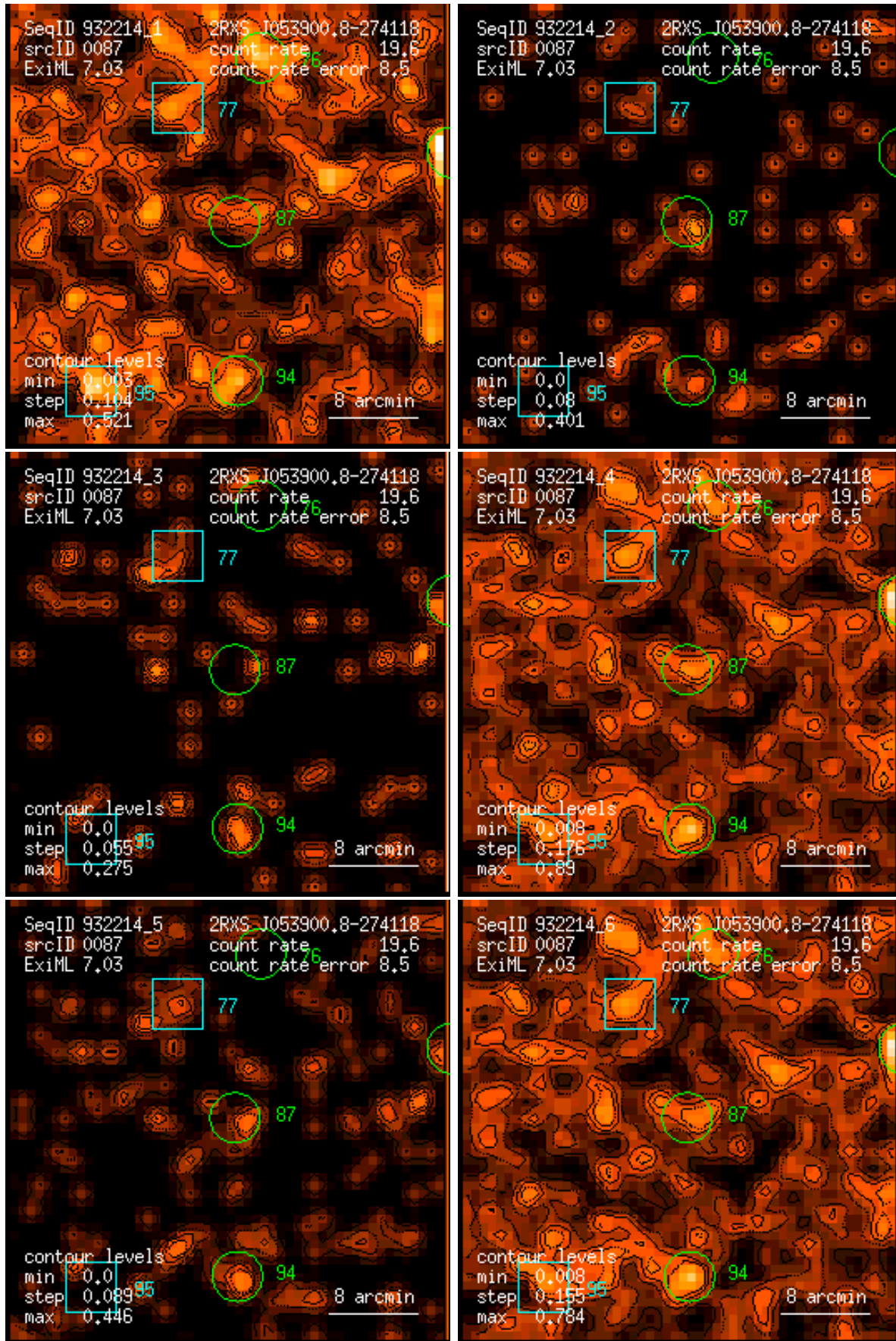
Figure 87: RASS 932214: detection 0087: band rate images, Gaussian filter: (1) PSPC channels 11 – 41, (2) 52 – 90, (3) 91 – 201, (4) 11 – 235, (5) 52 – 201, (6) 11 – 201. Broad band rates in counts/ks. Band rate contour levels in counts/ks/arcmin 2 .
