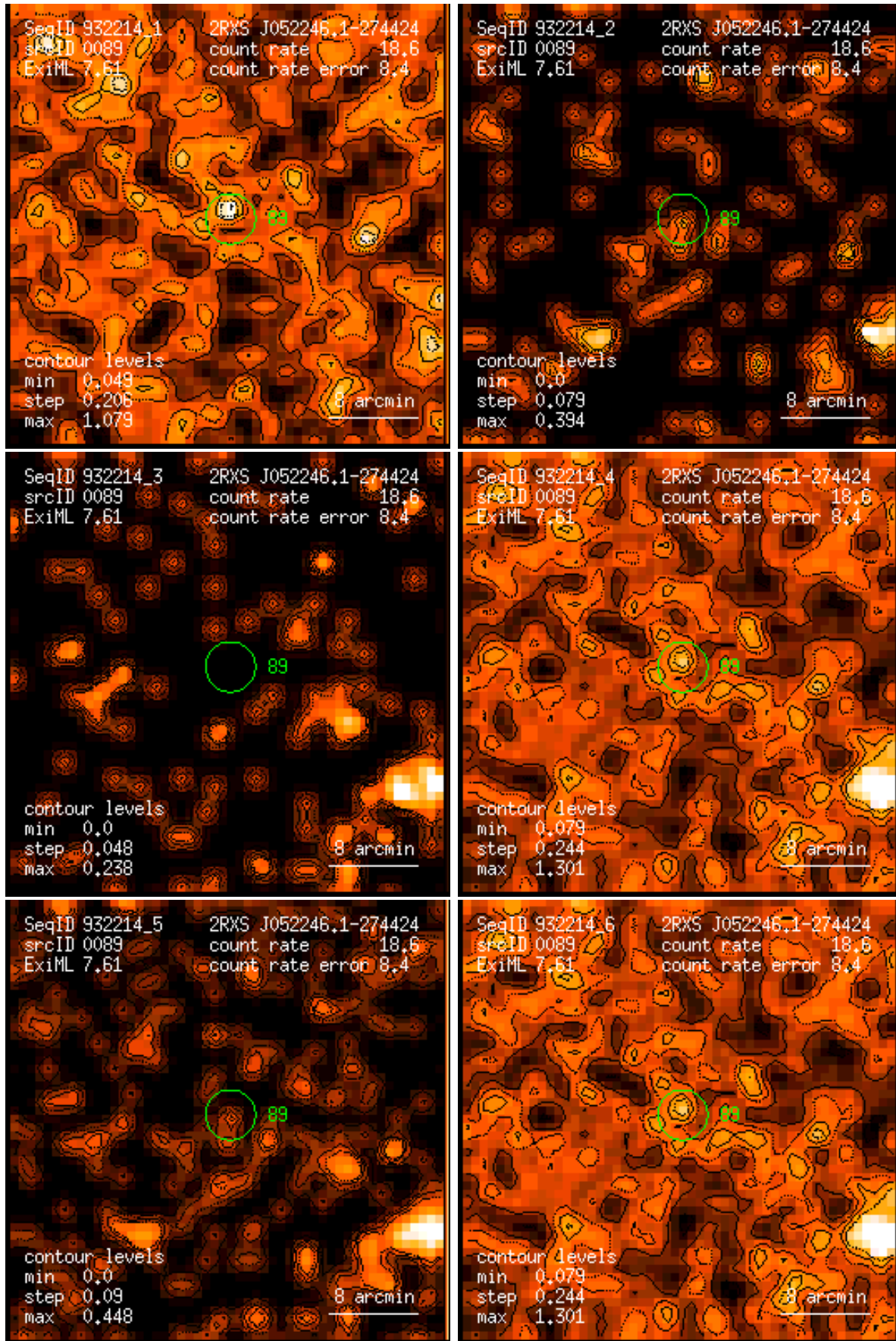
Figure 89: RASS 932214: detection 0089: band rate images, Gaussian filter: (1) PSPC channels 11 – 41, (2) 52 – 90, (3) 91 – 201, (4) 11 – 235, (5) 52 – 201, (6) 11 – 201. Broad band rates in counts/ks. Band rate contour levels in counts/ks/arcmin 2 .
