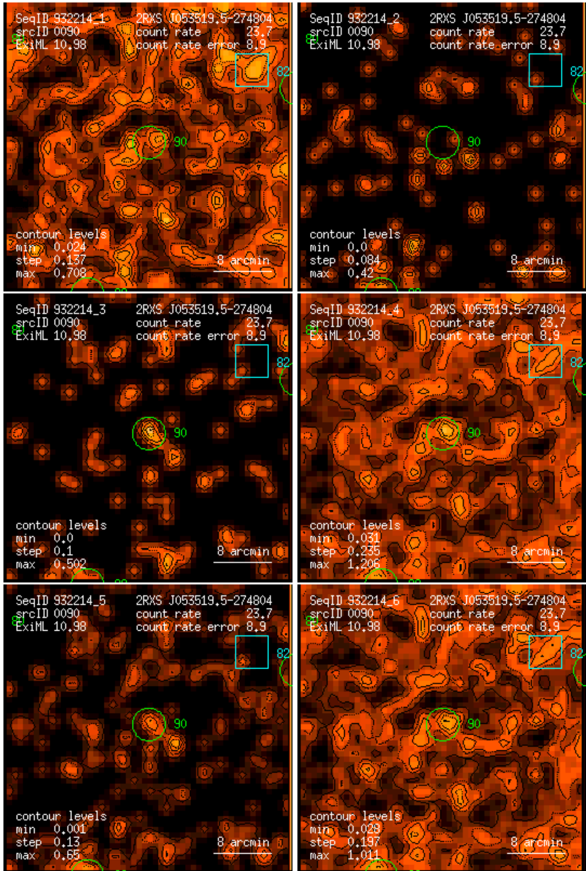
Figure 90: RASS 932214: detection 0090: band rate images, Gaussian filter: (1) PSPC channels 11 – 41, (2) 52 – 90, (3) 91 – 201, (4) 11 – 235, (5) 52 – 201, (6) 11 – 201. Broad band rates in counts/ks. Band rate contour levels in counts/ks/arcmin 2 .
