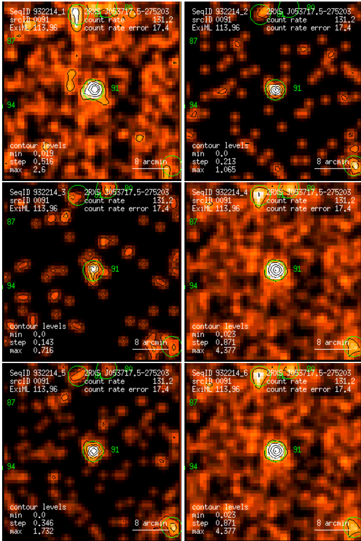
Figure 91: RASS 932214: detection 0091: band rate images, Gaussian filter: (1) PSPC channels 11 – 41, (2) 52 – 90, (3) 91 – 201, (4) 11 – 235, (5) 52 – 201, (6) 11 – 201. Broad band rates in counts/ks. Band rate contour levels in counts/ks/arcmin 2 .
