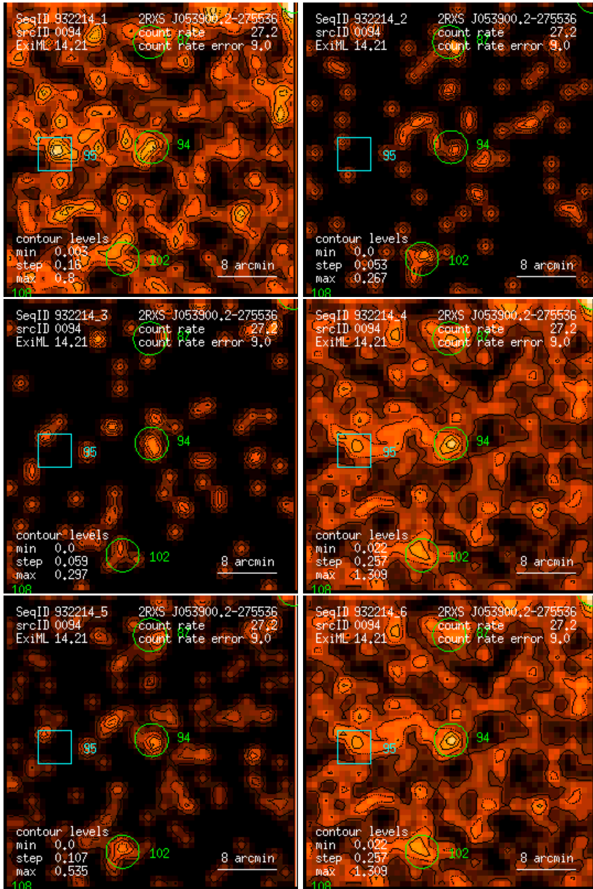
Figure 94: RASS 932214: detection 0094: band rate images, Gaussian filter: (1) PSPC channels 11 – 41, (2) 52 – 90, (3) 91 – 201, (4) 11 – 235, (5) 52 – 201, (6) 11 – 201. Broad band rates in counts/ks. Band rate contour levels in counts/ks/arcmin 2 .
