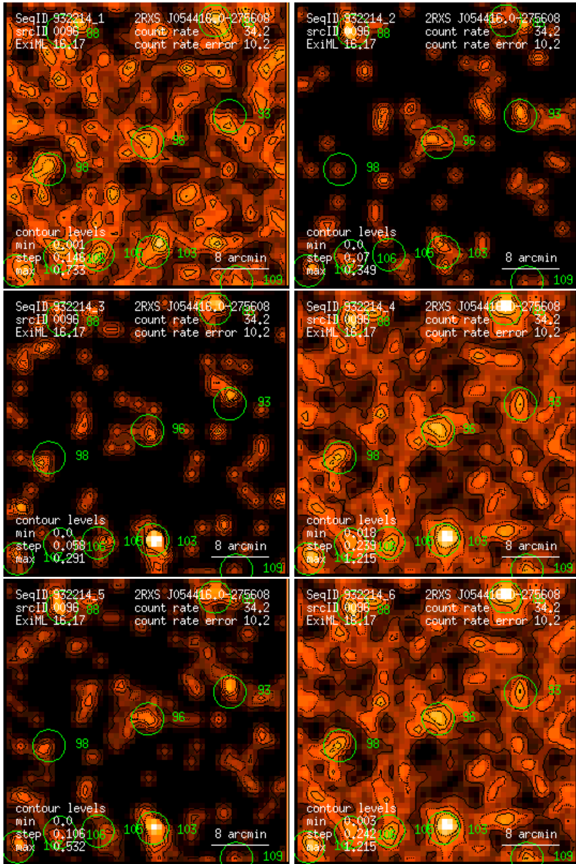
Figure 96: RASS 932214: detection 0096: band rate images, Gaussian filter: (1) PSPC channels 11 – 41, (2) 52 – 90, (3) 91 – 201, (4) 11 – 235, (5) 52 – 201, (6) 11 – 201. Broad band rates in counts/ks. Band rate contour levels in counts/ks/arcmin 2 .
