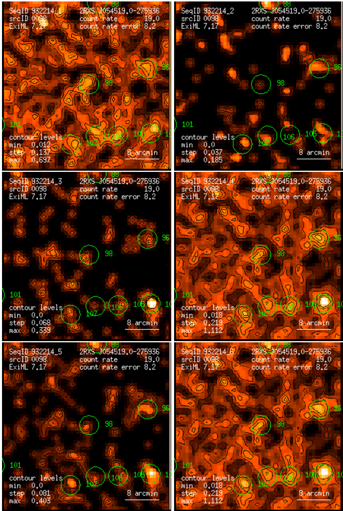
Figure 98: RASS 932214: detection 0098: band rate images, Gaussian filter: (1) PSPC channels 11 – 41, (2) 52 – 90, (3) 91 – 201, (4) 11 – 235, (5) 52 – 201, (6) 11 – 201. Broad band rates in counts/ks. Band rate contour levels in counts/ks/arcmin 2 .
