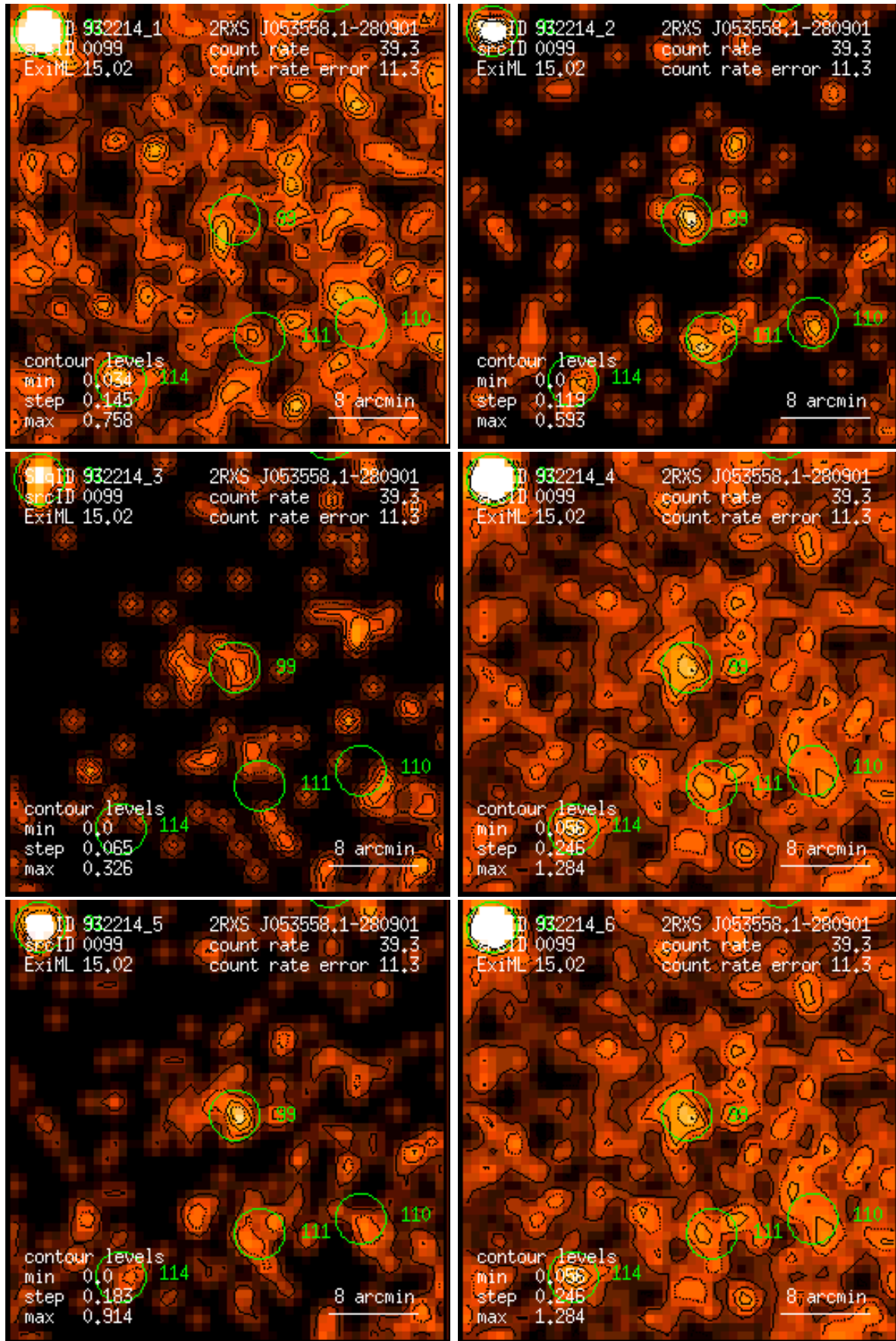
Figure 99: RASS 932214: detection 0099: band rate images, Gaussian filter: (1) PSPC channels 11 – 41, (2) 52 – 90, (3) 91 – 201, (4) 11 – 235, (5) 52 – 201, (6) 11 – 201. Broad band rates in counts/ks. Band rate contour levels in counts/ks/arcmin 2 .
