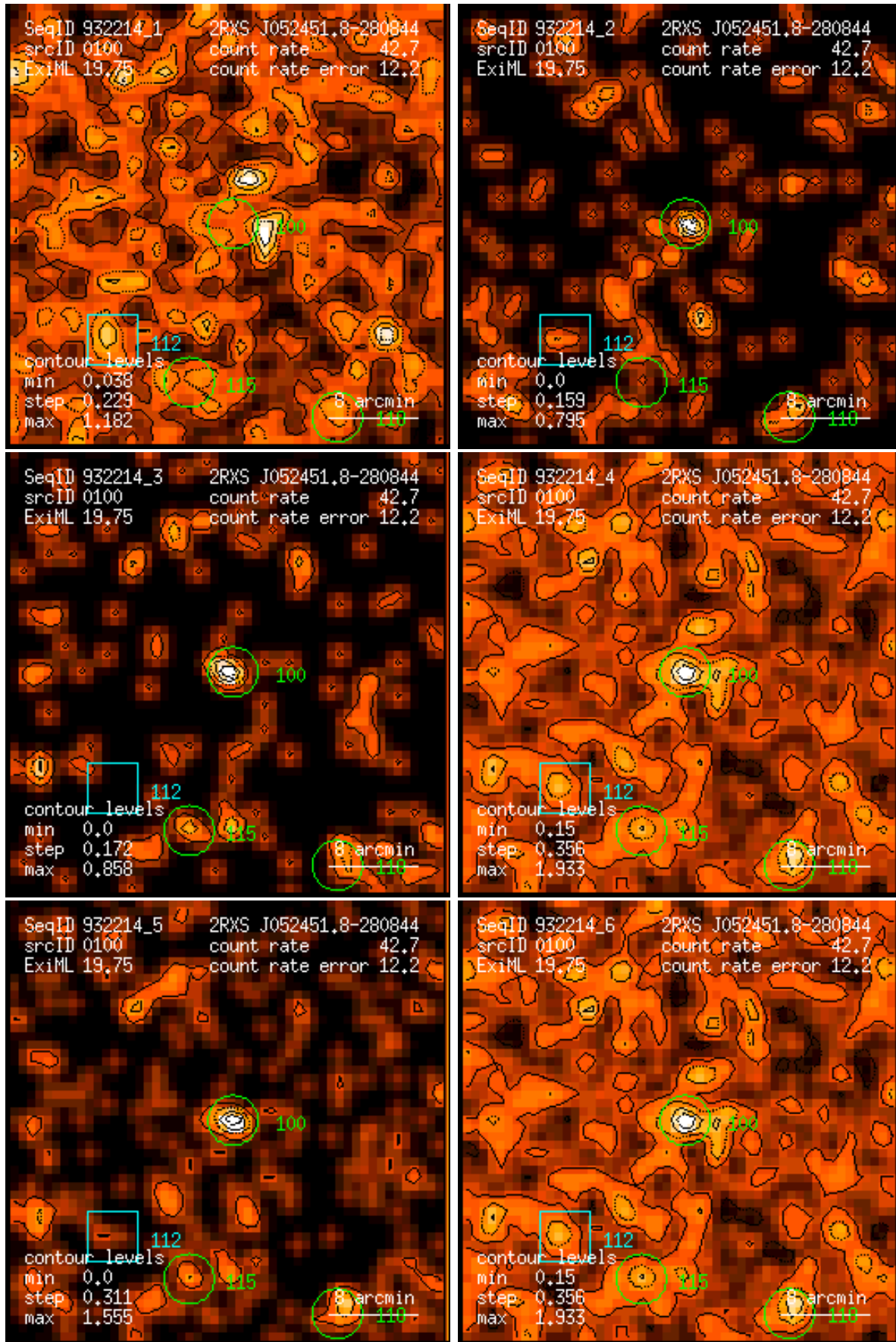
Figure 100: RASS 932214: detection 0100: band rate images, Gaussian filter: (1) PSPC channels 11 – 41, (2) 52 – 90, (3) 91 – 201, (4) 11 – 235, (5) 52 – 201, (6) 11 – 201. Broad band rates in counts/ks. Band rate contour levels in counts/ks/arcmin 2 .
