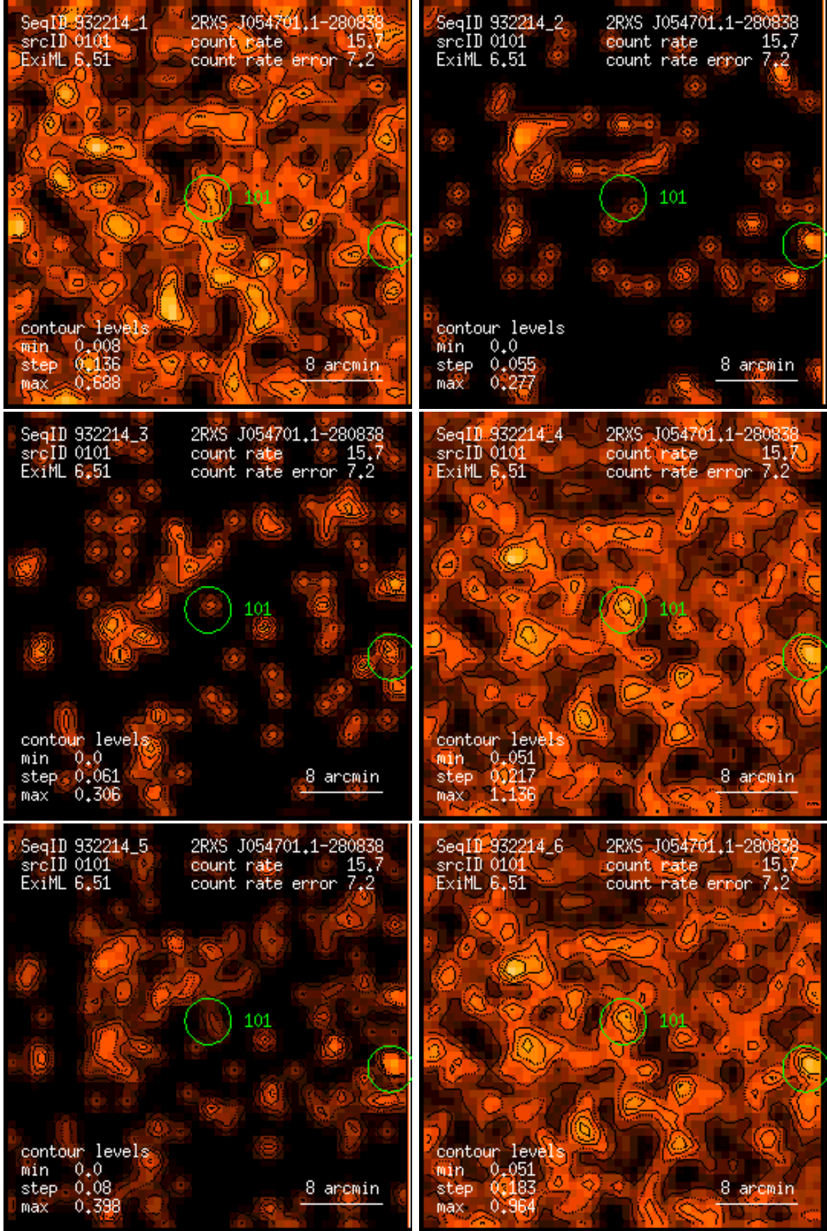
Figure 101: RASS 932214: detection 0101: band rate images, Gaussian filter: (1) PSPC channels 11 – 41, (2) 52 – 90, (3) 91 – 201, (4) 11 – 235, (5) 52 – 201, (6) 11 – 201. Broad band rates in counts/ks. Band rate contour levels in counts/ks/arcmin 2 .
