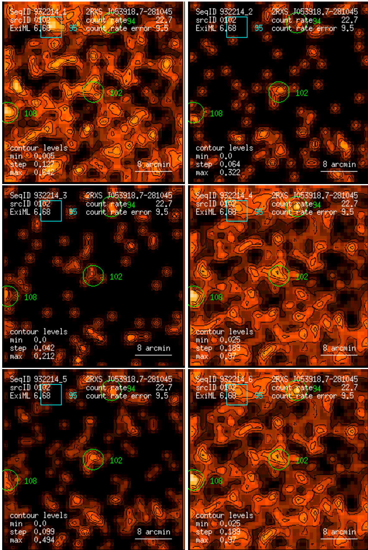
Figure 102: RASS 932214: detection 0102: band rate images, Gaussian filter: (1) PSPC channels 11 – 41, (2) 52 – 90, (3) 91 – 201, (4) 11 – 235, (5) 52 – 201, (6) 11 – 201. Broad band rates in counts/ks. Band rate contour levels in counts/ks/arcmin 2 .
