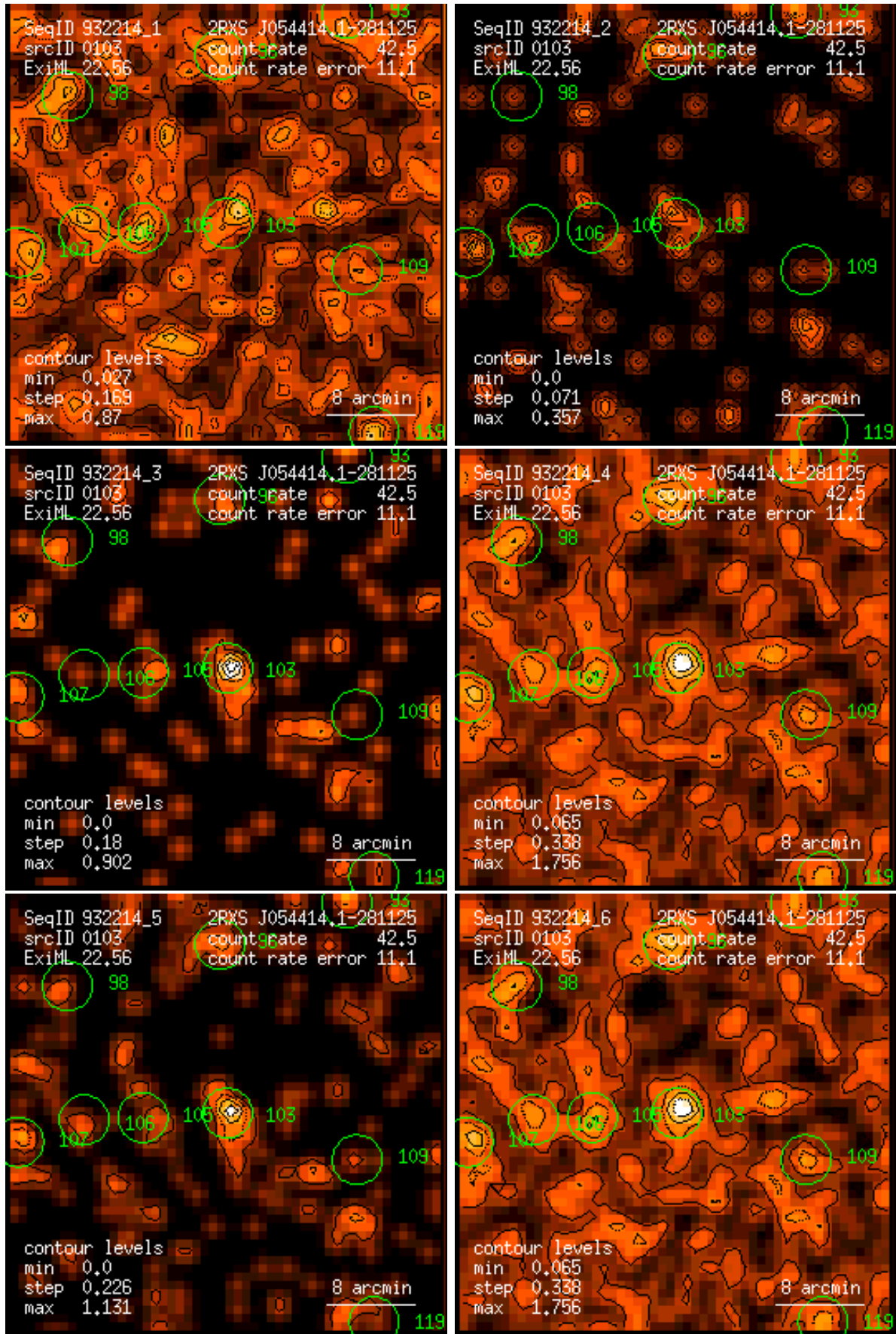
Figure 103: RASS 932214: detection 0103: band rate images, Gaussian filter: (1) PSPC channels 11 – 41, (2) 52 – 90, (3) 91 – 201, (4) 11 – 235, (5) 52 – 201, (6) 11 – 201. Broad band rates in counts/ks. Band rate contour levels in counts/ks/arcmin 2 .
