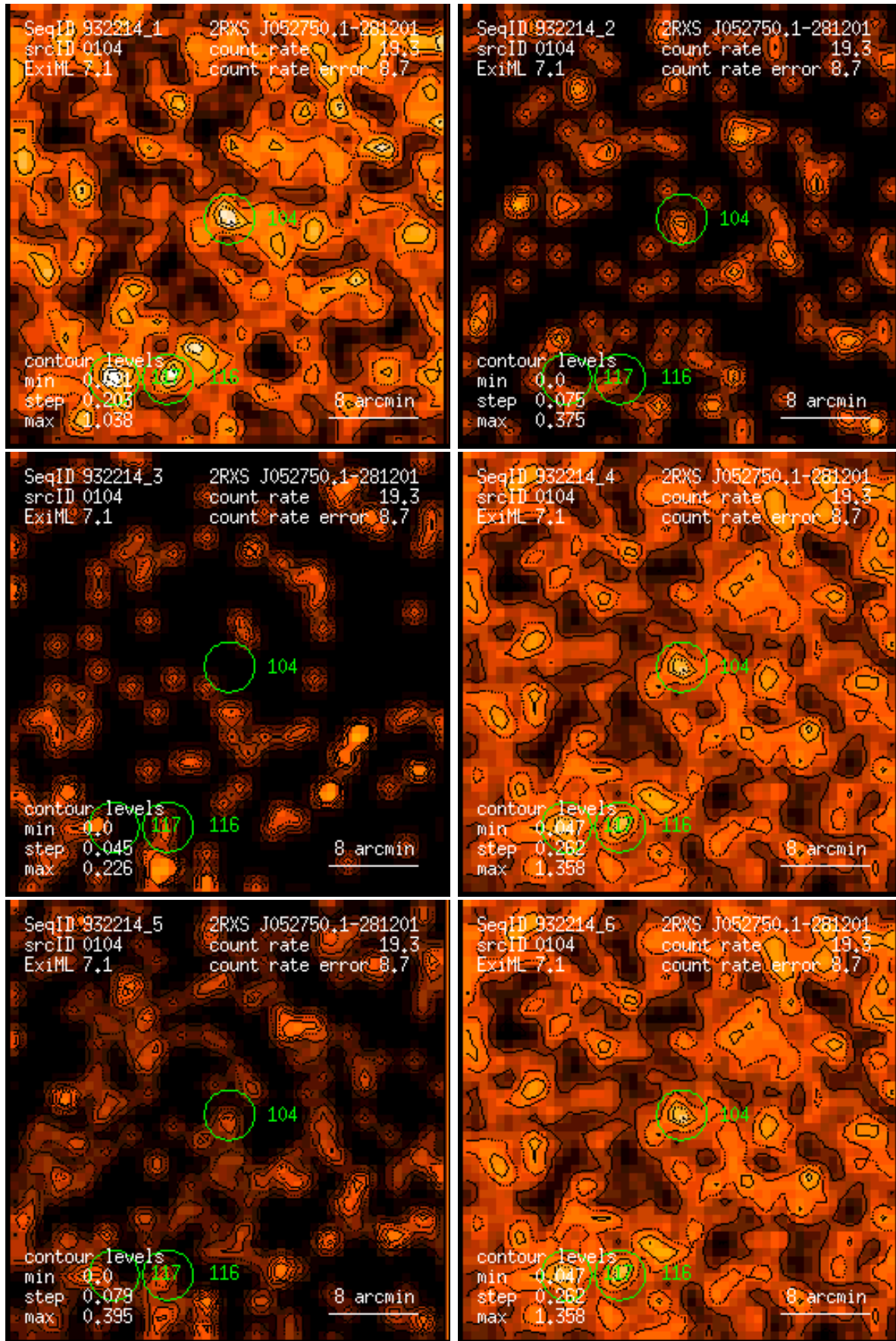
Figure 104: RASS 932214: detection 0104: band rate images, Gaussian filter: (1) PSPC channels 11 – 41, (2) 52 – 90, (3) 91 – 201, (4) 11 – 235, (5) 52 – 201, (6) 11 – 201. Broad band rates in counts/ks. Band rate contour levels in counts/ks/arcmin 2 .
