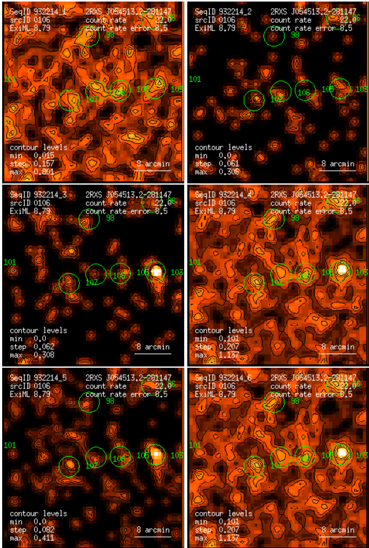
Figure 106: RASS 932214: detection 0106: band rate images, Gaussian filter: (1) PSPC channels 11 – 41, (2) 52 – 90, (3) 91 – 201, (4) 11 – 235, (5) 52 – 201, (6) 11 – 201. Broad band rates in counts/ks. Band rate contour levels in counts/ks/arcmin 2 .
