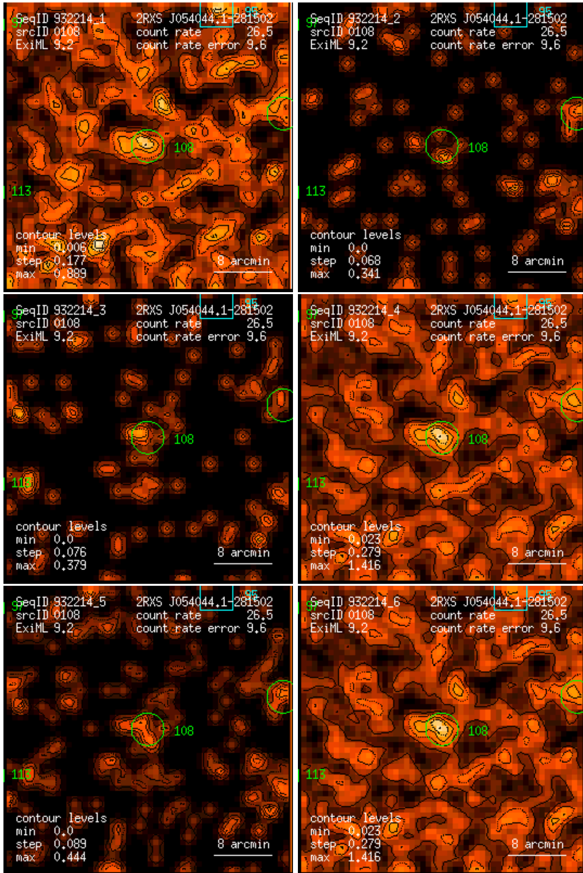
Figure 108: RASS 932214: detection 0108: band rate images, Gaussian filter: (1) PSPC channels 11 – 41, (2) 52 – 90, (3) 91 – 201, (4) 11 – 235, (5) 52 – 201, (6) 11 – 201. Broad band rates in counts/ks. Band rate contour levels in counts/ks/arcmin 2 .
