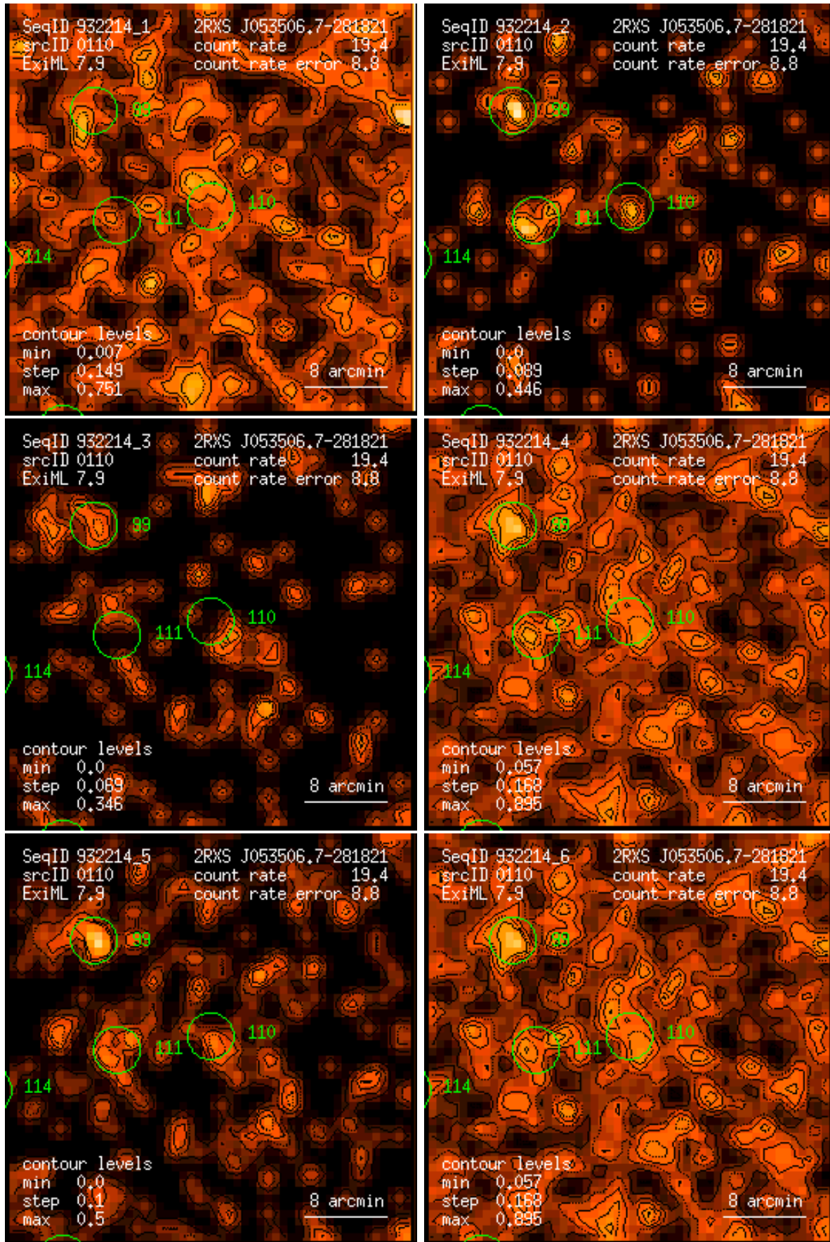
Figure 110: RASS 932214: detection 0110: band rate images, Gaussian filter: (1) PSPC channels 11 – 41, (2) 52 – 90, (3) 91 – 201, (4) 11 – 235, (5) 52 – 201, (6) 11 – 201. Broad band rates in counts/ks. Band rate contour levels in counts/ks/arcmin 2 .
