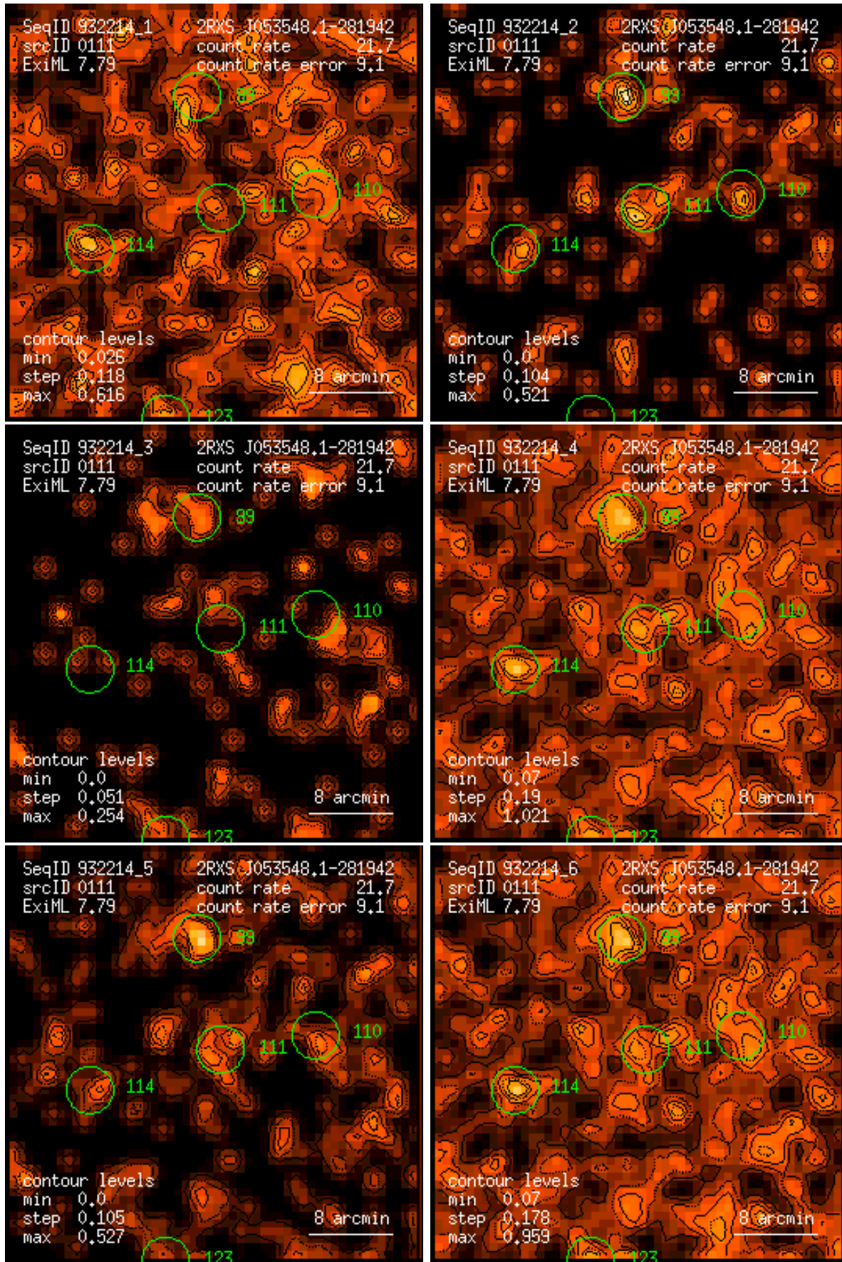
Figure 111: RASS 932214: detection 0111: band rate images, Gaussian filter: (1) PSPC channels 11 – 41, (2) 52 – 90, (3) 91 – 201, (4) 11 – 235, (5) 52 – 201, (6) 11 – 201. Broad band rates in counts/ks. Band rate contour levels in counts/ks/arcmin 2 .
